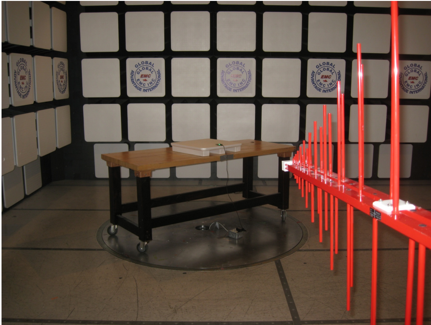
Radiated Emissions – Photo 1
