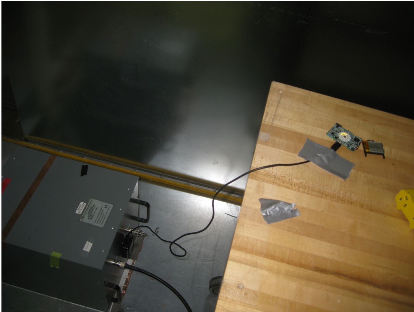
Power Line Conducted Emissions – Photo 1
