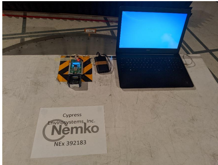
Figure 4 - Radiated emissions test setup, 30 - 1000 MHz, front
