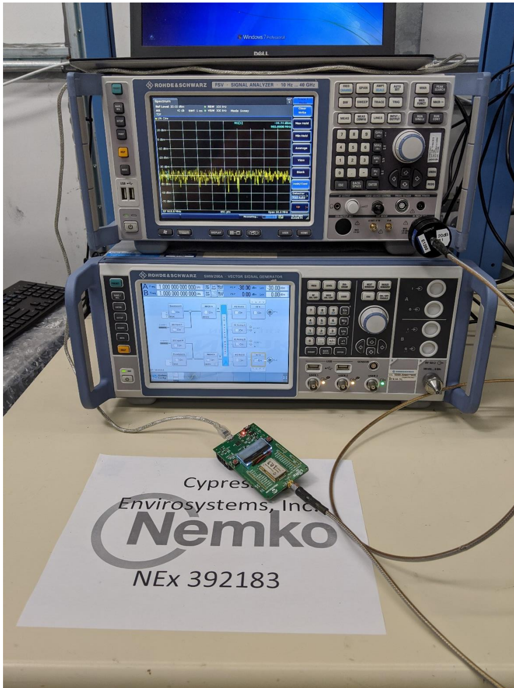
Figure 1 - Antenna port conducted measurement test setup
