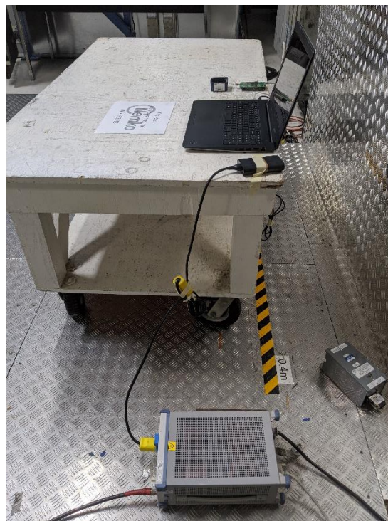
Figure 3 - AC conducted emissions test setup - side
