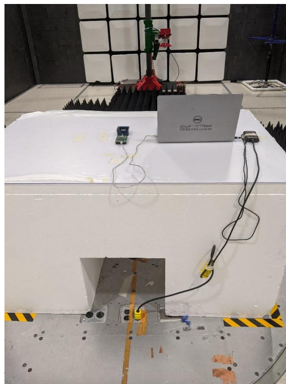
Figure 6 – Unintentional Radiated emissions test setup, 1 - 18 GHz, front
