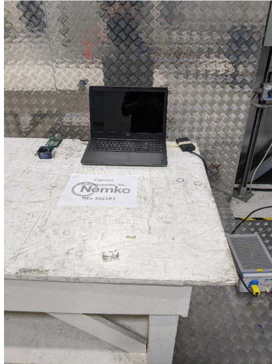
Figure 2 - AC conducted emissions test setup - front
