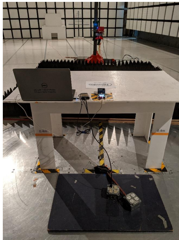
Figure 5 - Radiated emissions test setup, 30 - 1000 MHz, back
