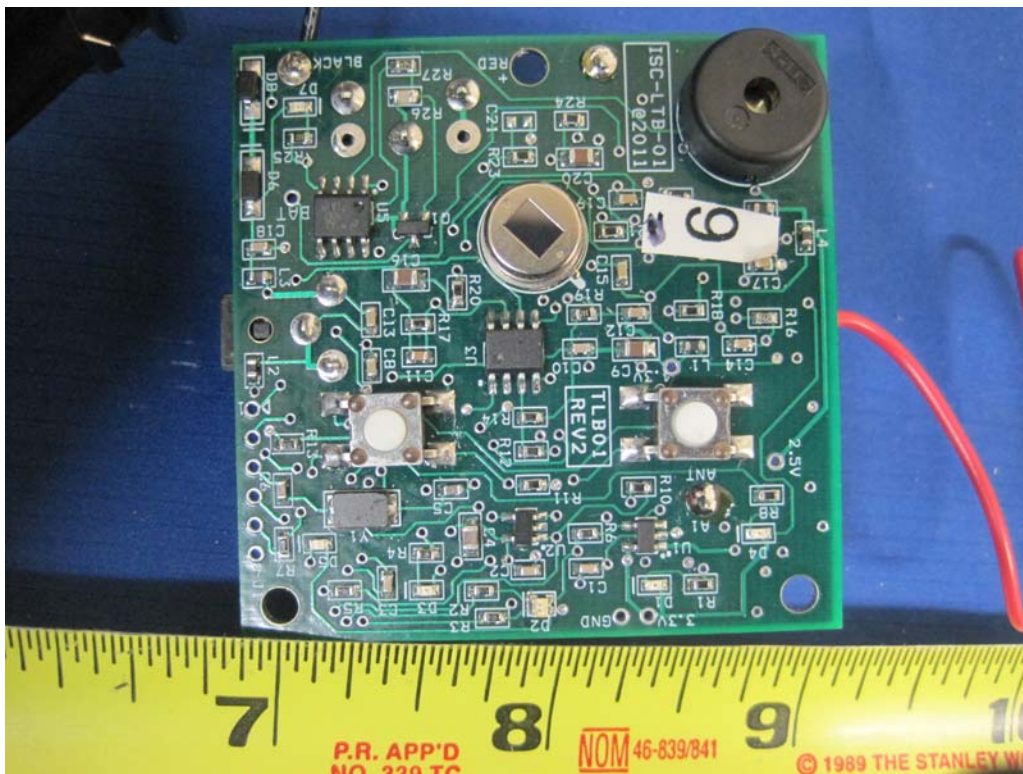
PCBA board Bottom View
