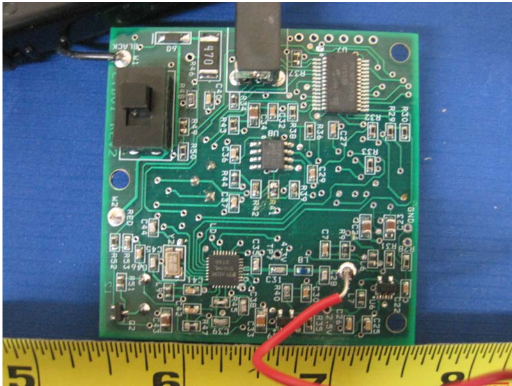
PCBA board Top View
