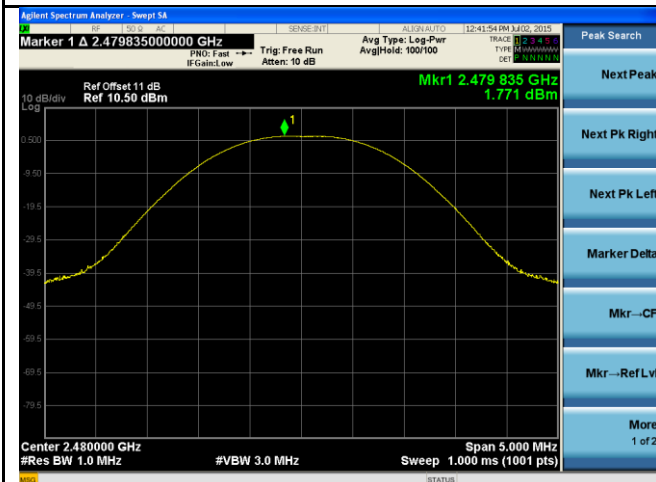
Output power - High CH 2480 - Basic data rate
