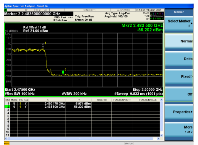
Band Edge-Hopping-EDR High
