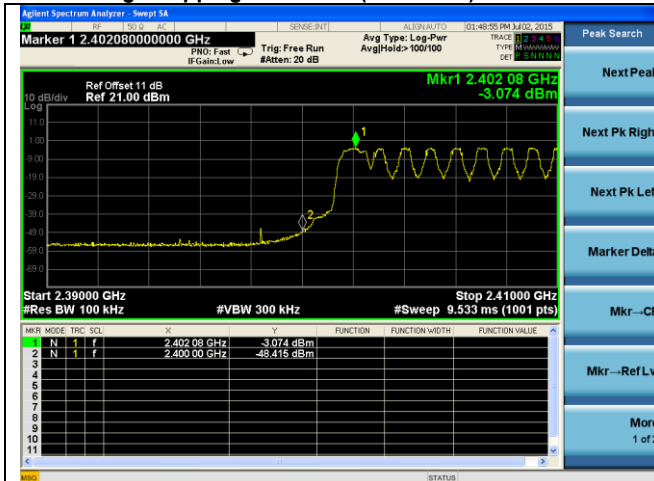
Band Edge-Hopping-BDR Low
