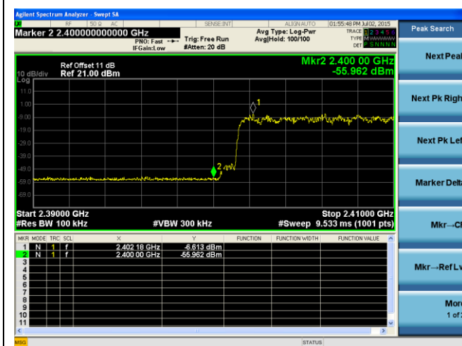
Band Edge-Hopping-EDR Low
