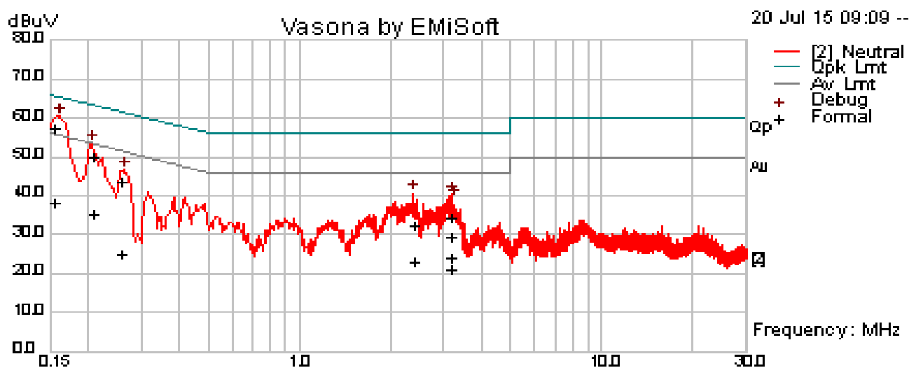
Neutral Line Plot @ 120Vac, 60Hz
