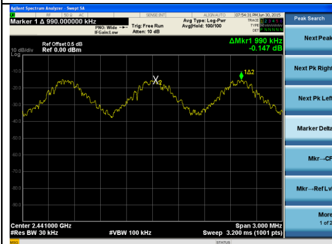
Channel Separation-Mid Channel-BDR Mode
