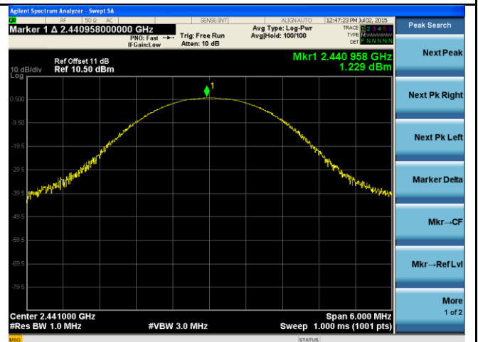
Output power - Mid CH 2441 - Enhanced data rate
