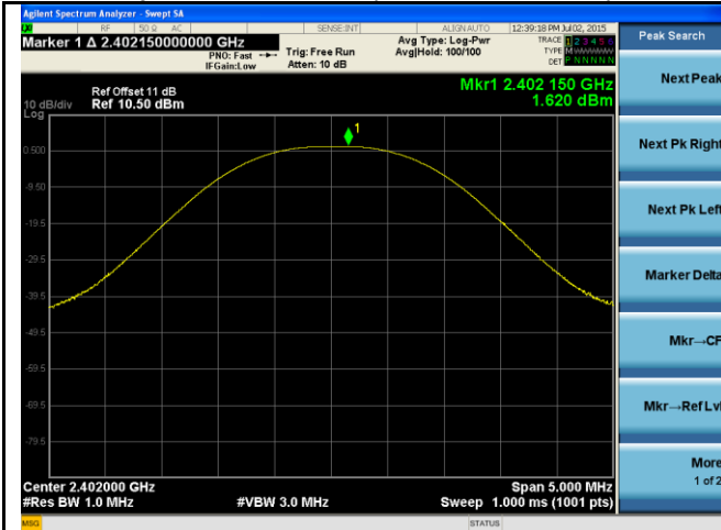
Output power - Low CH 2402 - Basic data rate
