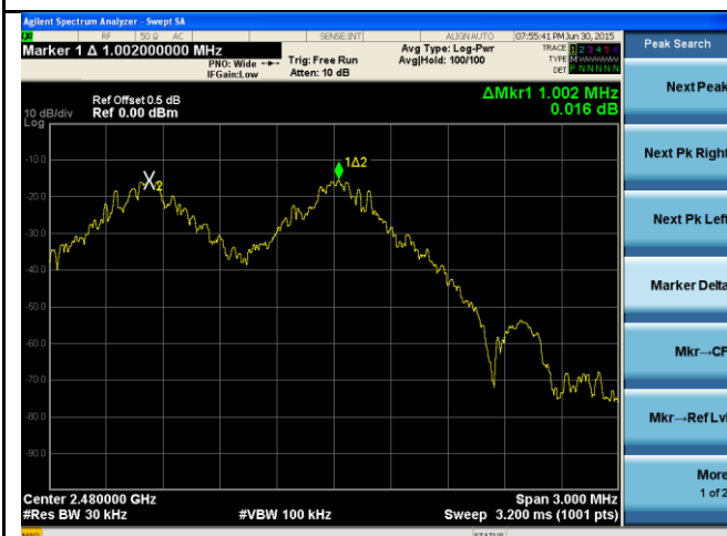
Channel Separation-High Channel-BDR Mode
