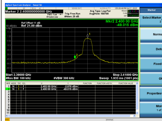
Band Edge-Single-EDR Low
