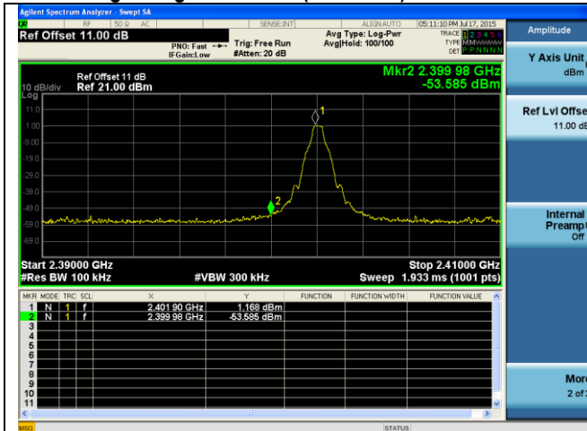
Band Edge-Single-BDR Low
