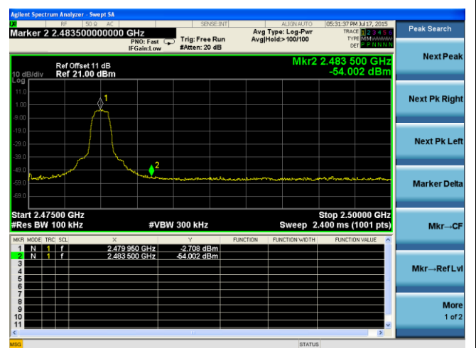
Band Edge-Single-EDR High
