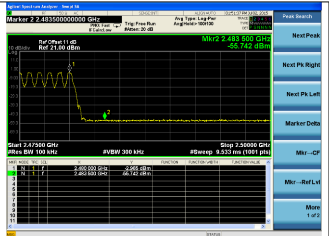
Band Edge-Hopping-BDR High
