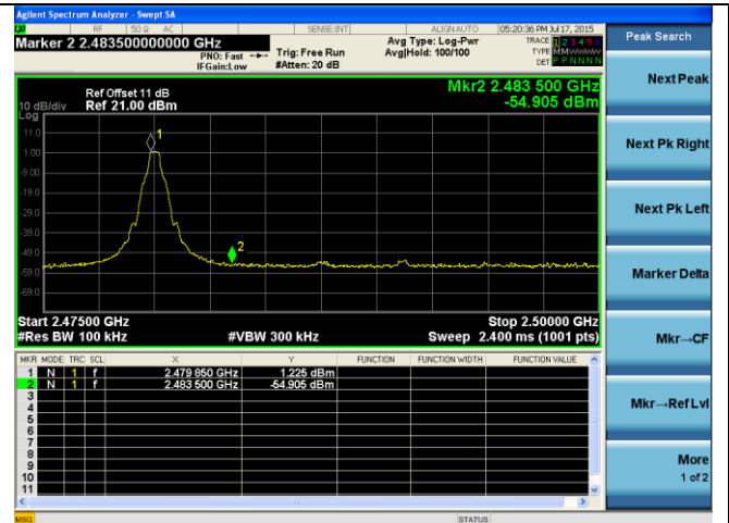
Band Edge-Single-BDR High
