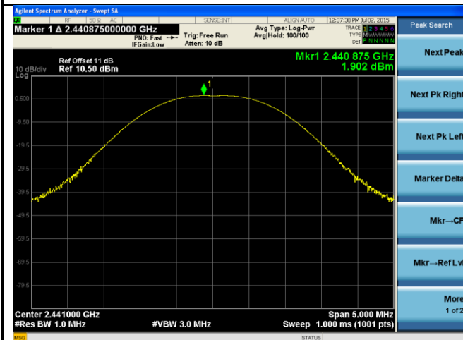
Output power - Mid CH 2441 - Basic data rate
