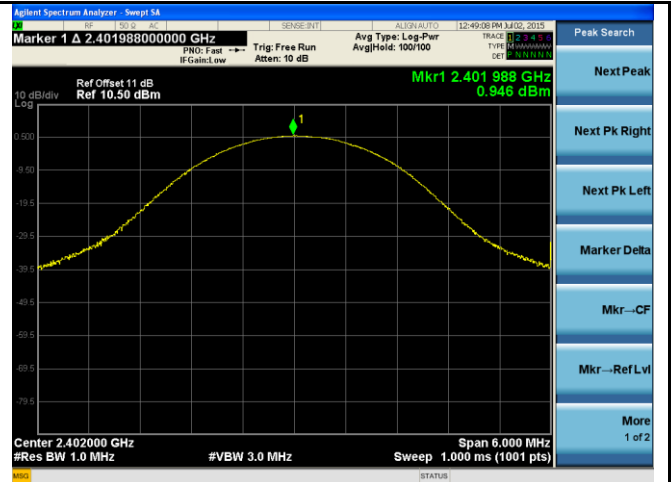
Output power - Low CH 2402 - Enhanced data rate
