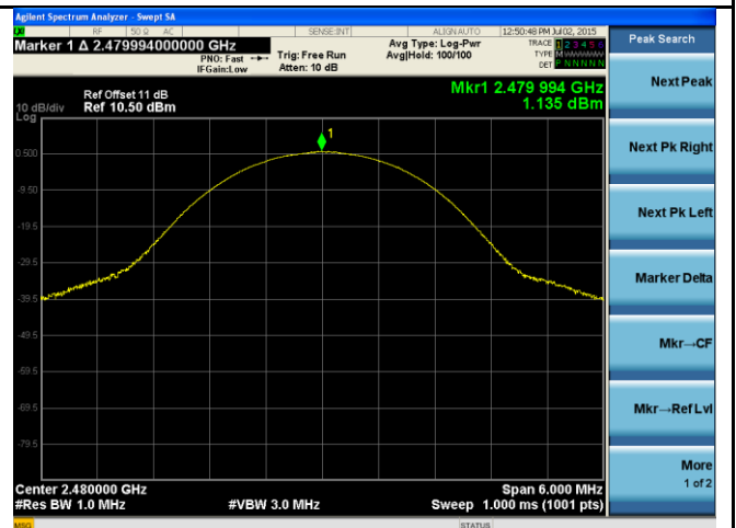
Output power - High CH 2480 - Enhanced data rate
