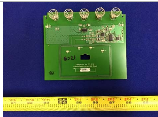
EUT-RFID Board with antenna Front View
