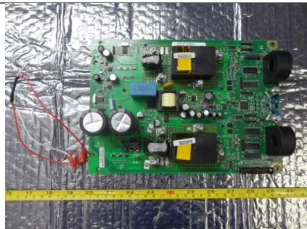
PCBA – Power Supply Top View
