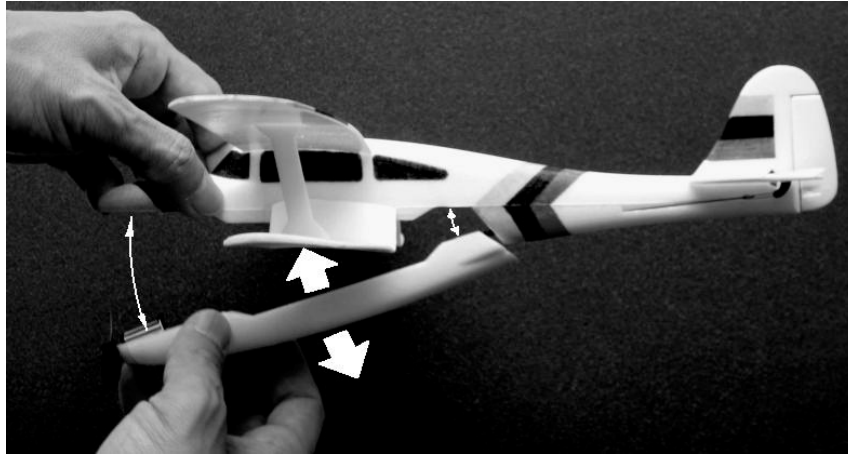
Photo 2C1. – Hinge the Base Module to connect to the airplane module
