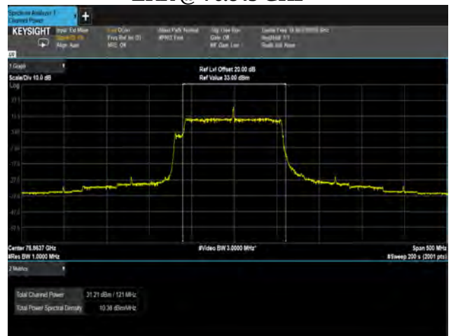
LRR @ 76.845 GHz
