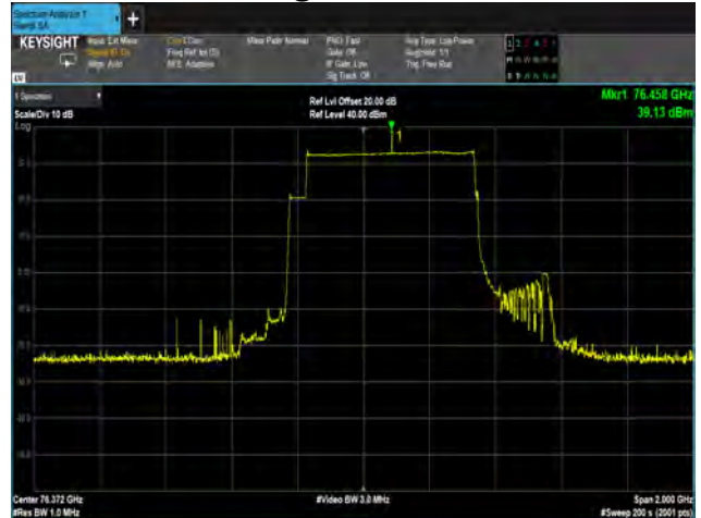
MRR @ 76.458 GHz
