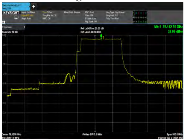
LRR @ 76.143 GHz
