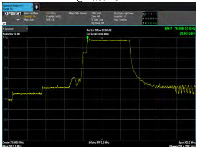
LRR @ 76.807 GHz
