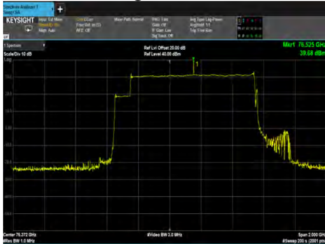
SRR @ 76.525 GHz
