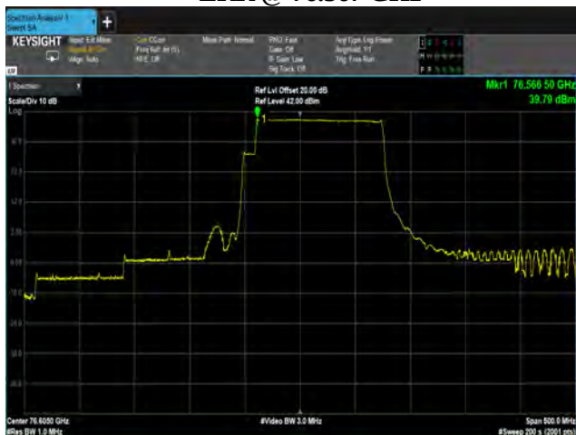
LRR @ 76.567 GHz
