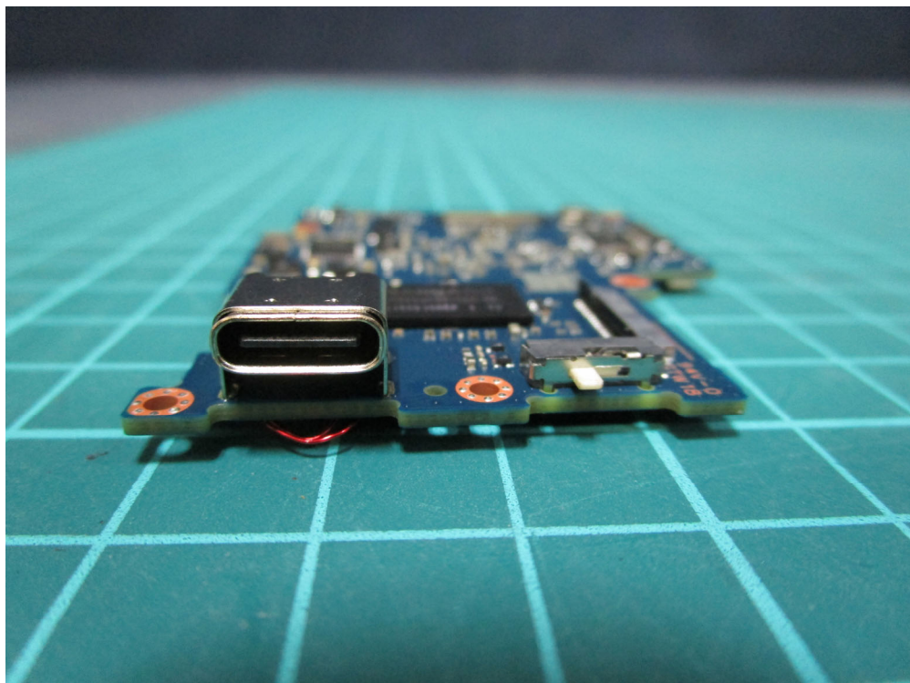
(55) EUT Photo
