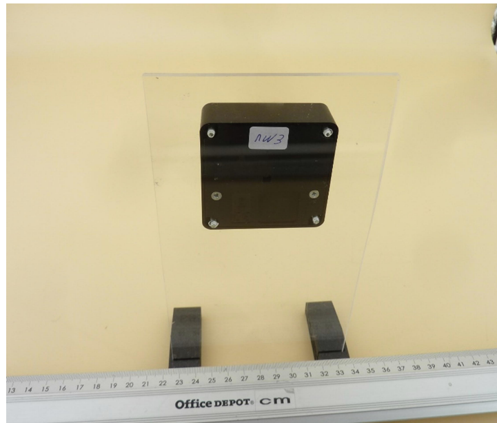
201474_eut05: Front view EUT in Setup A
