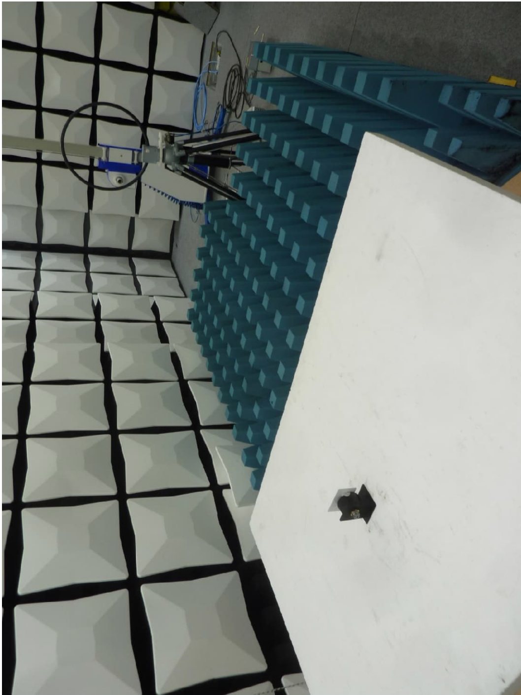
Test setup fully-anechoic chamber M154; Preliminary measurement 9 kHz to 30 MHz
