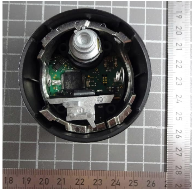
EUT, housing opened
