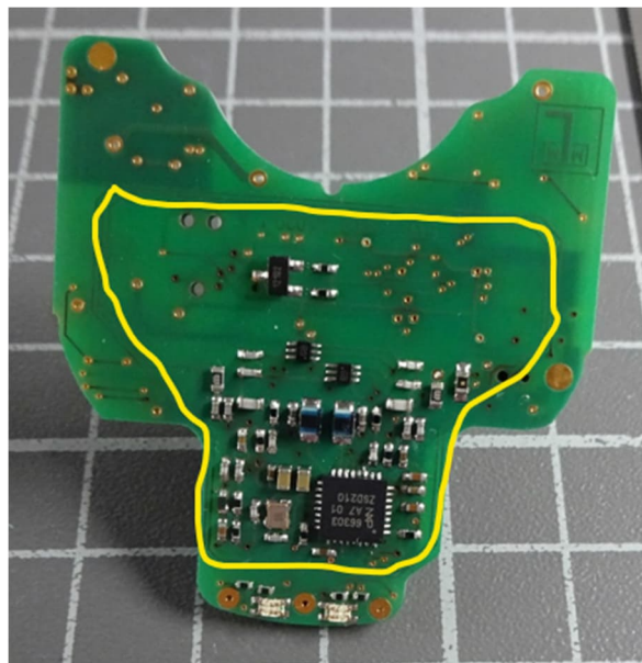
13.56 MHz Antenna
