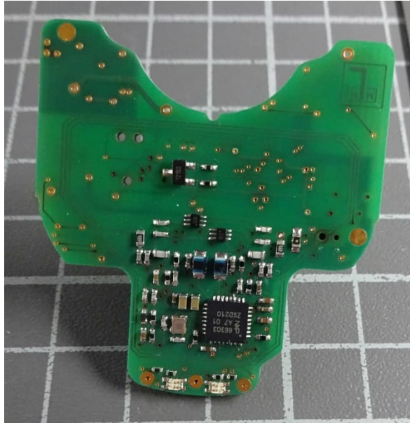
PCB, bottom view
