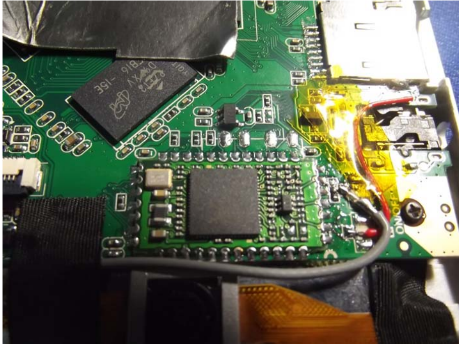
Figure 9 PCB of the EUT-Module View
