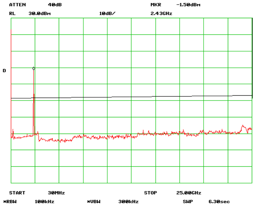
Antenna Port Emission Mid Channel (802.11g)
