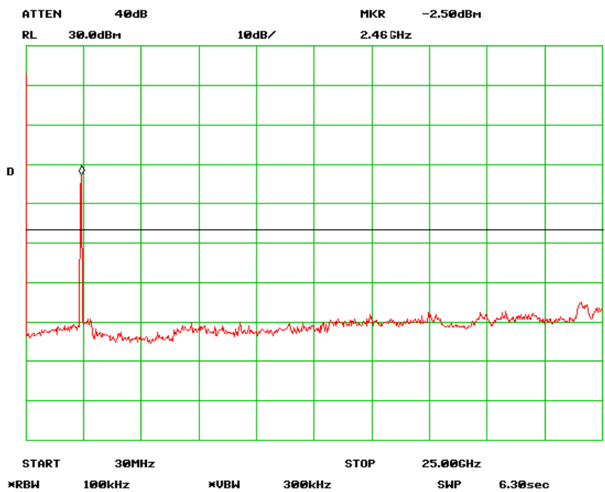
Antenna Port Emission High Channel (802.11g)
