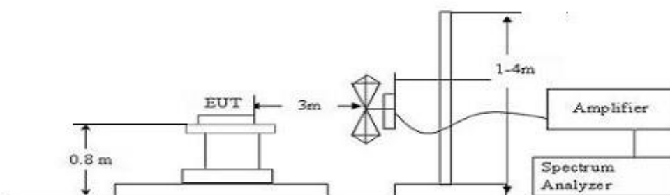
Block Diagram of test setup (above 30MHz)
