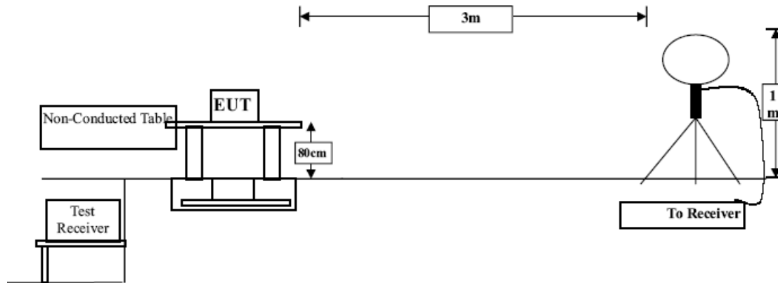
Block Diagram of test setup (below 30MHz)
