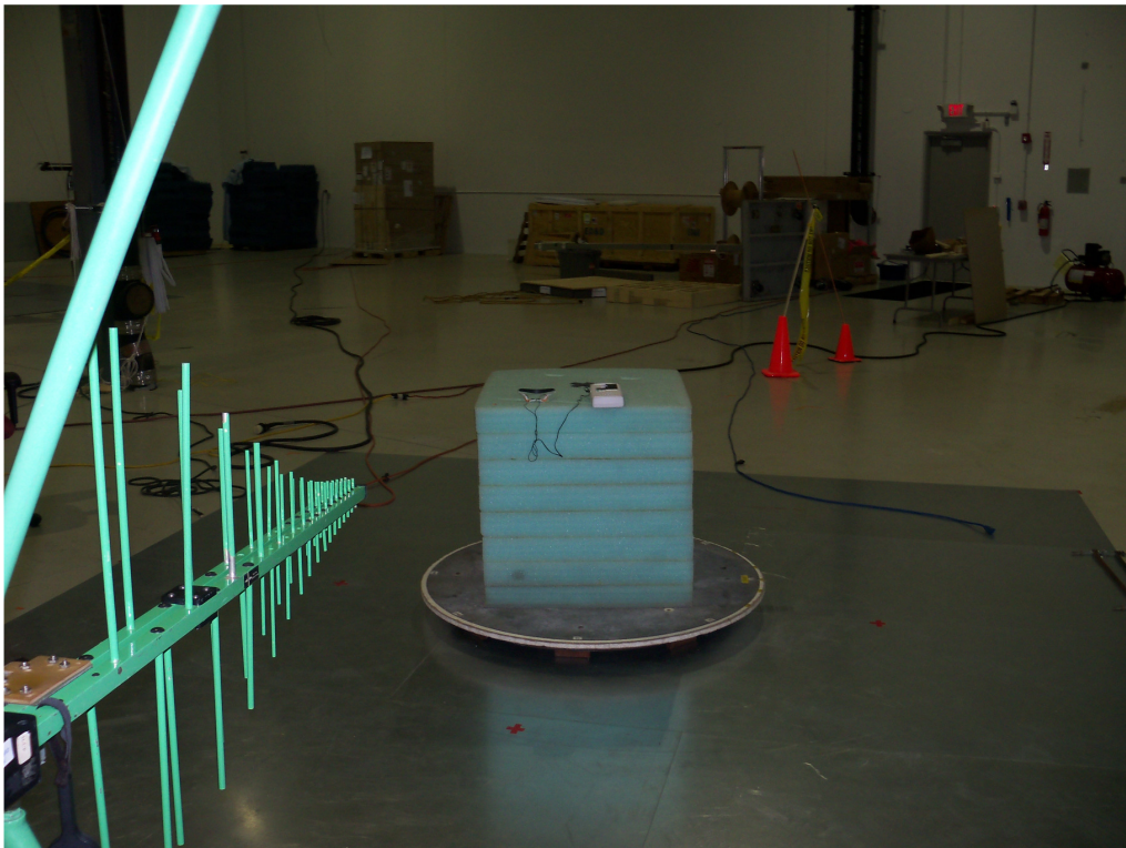
Radiated Emissions above 30MHz
