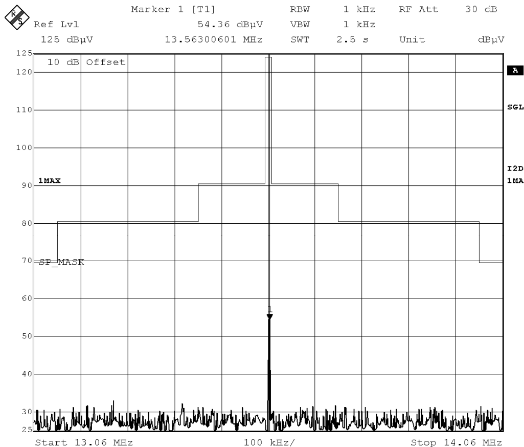
Figure 6: Spectrum Mask
