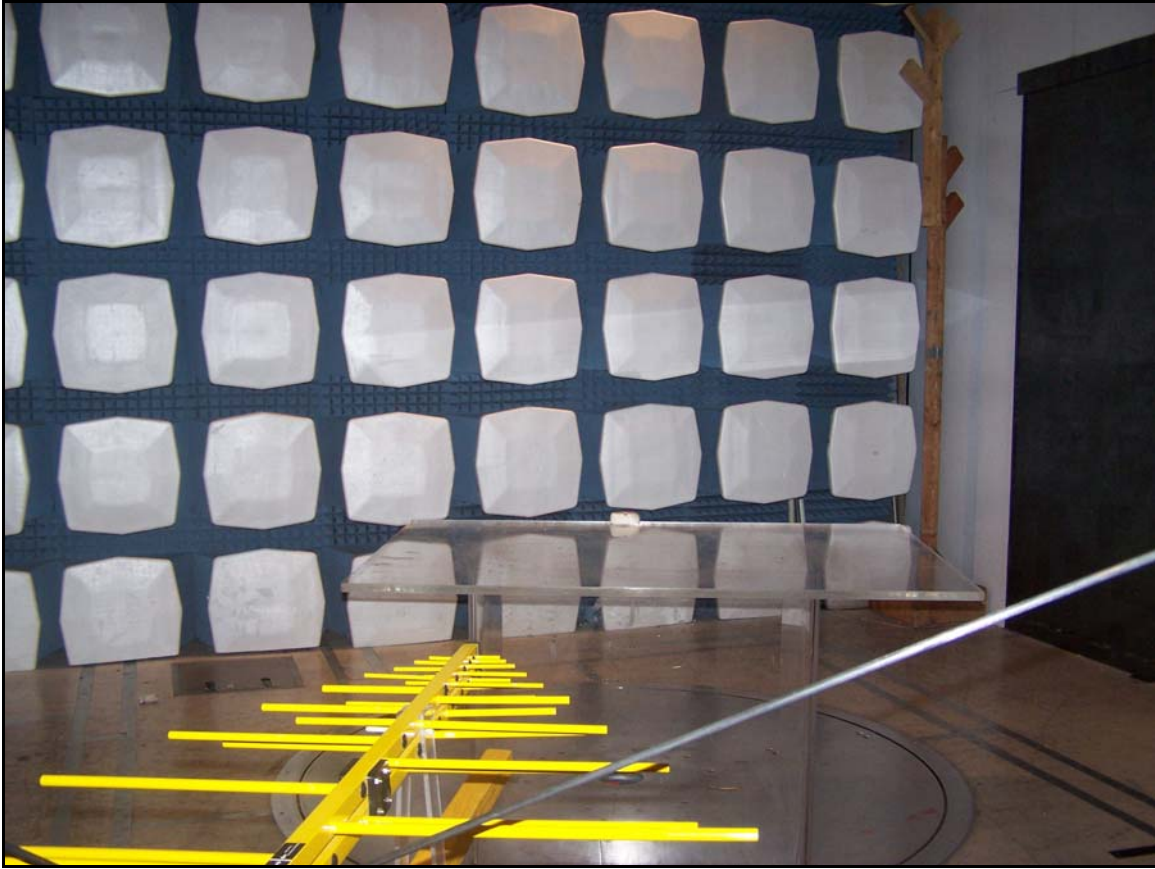
Photograph 1. BarMate System, SRD, Test Setup
