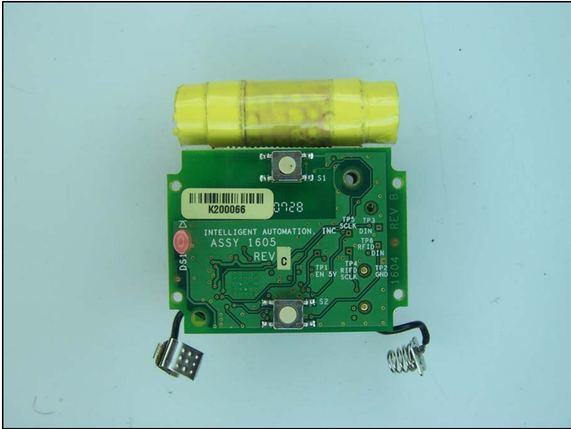
Photograph 3. BarMate System, SRD
