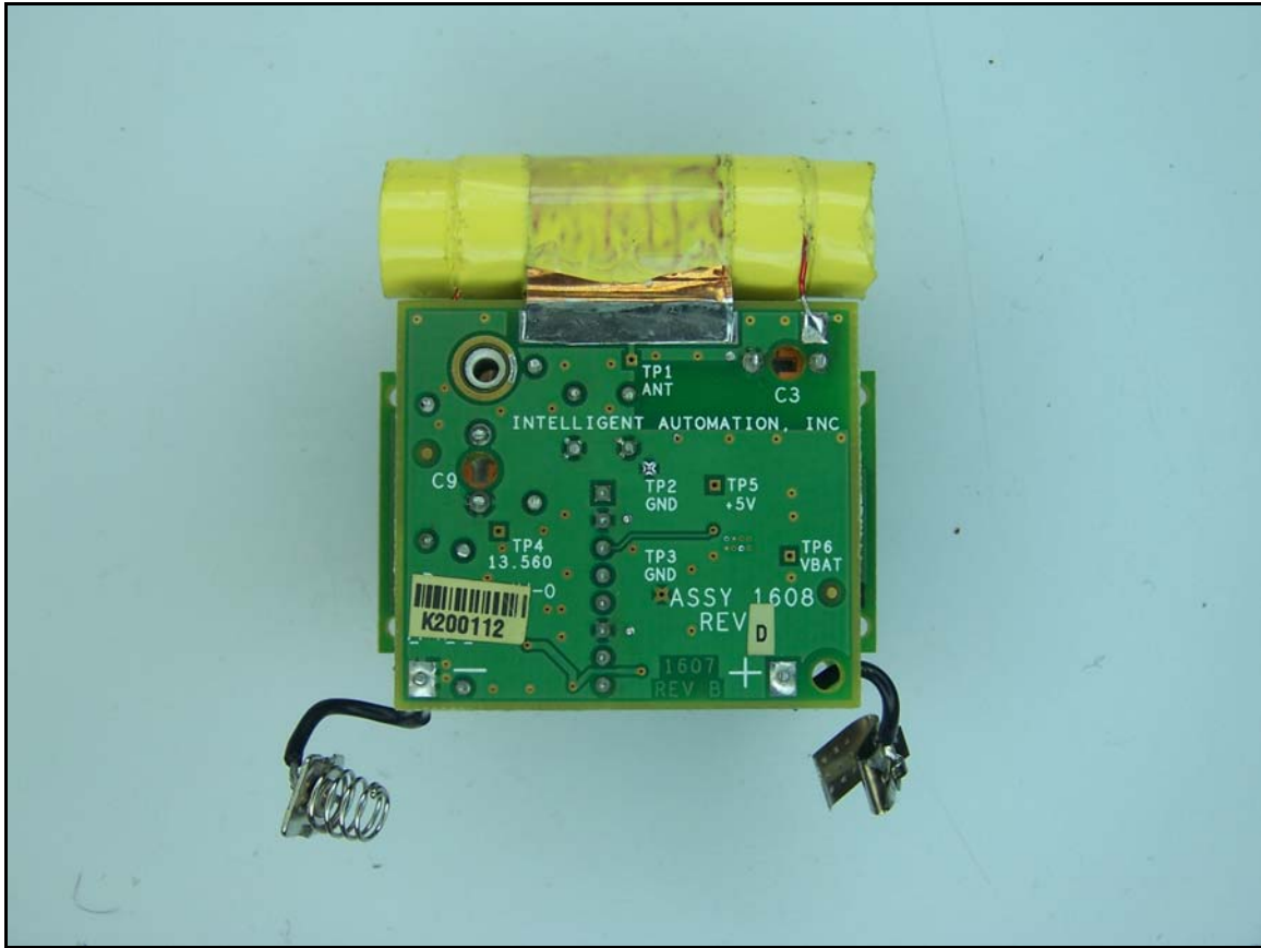
Photograph 2. BarMate System, SRD
