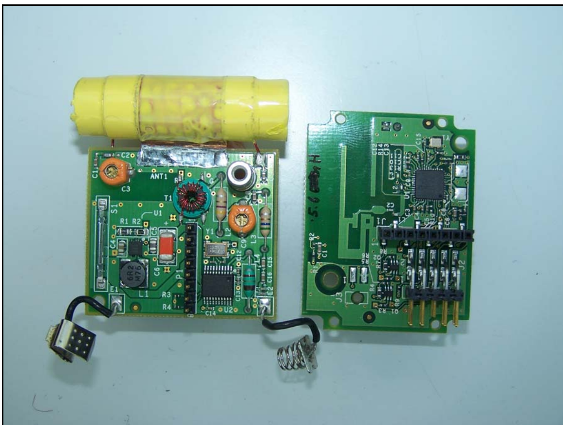
Photograph 4. BarMate System, SRD
