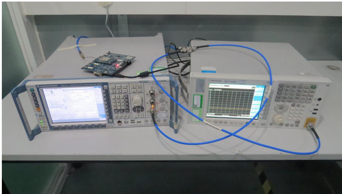
Conduct test setup
