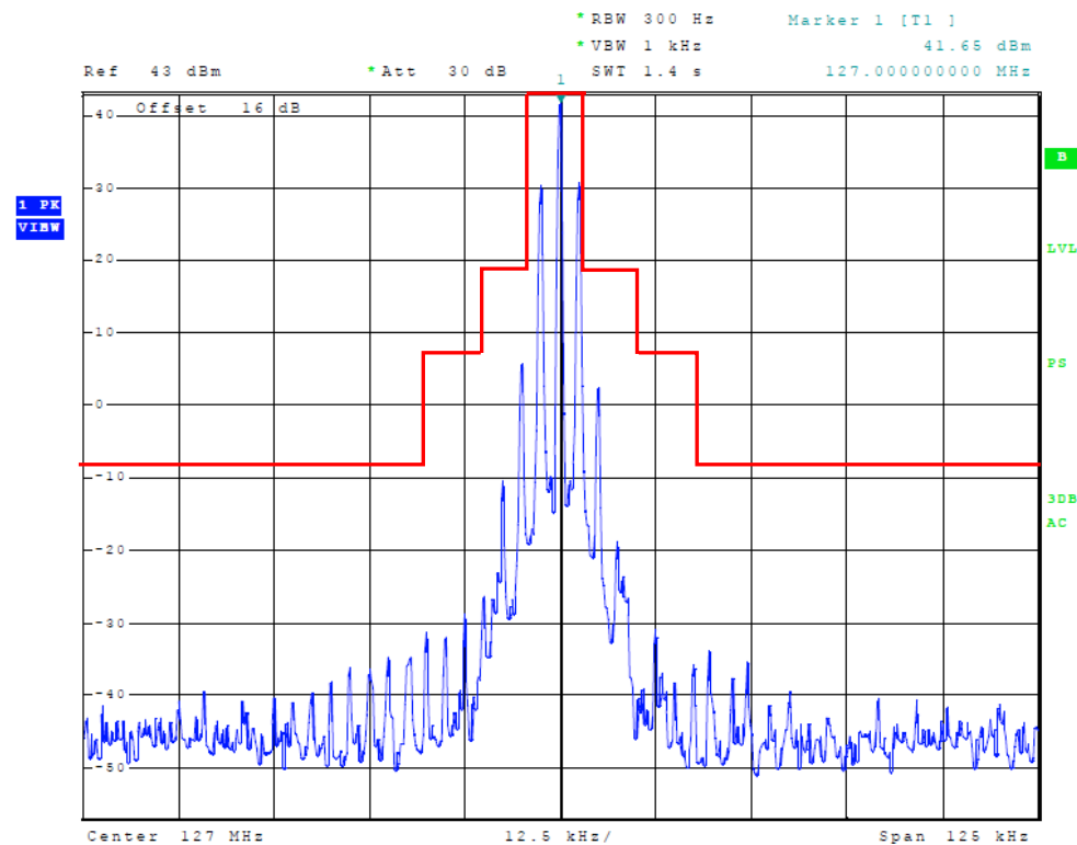
Figure 10 Emission Mask
