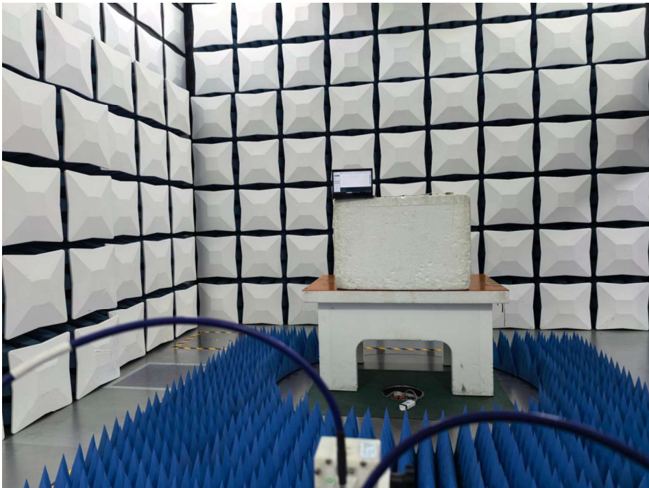
Test Set-up: Radiated spurious emission 18GHz to 25GHz
