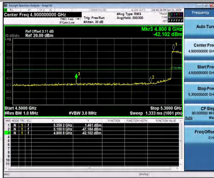
11AX80SISO_Ant1_High_5290
