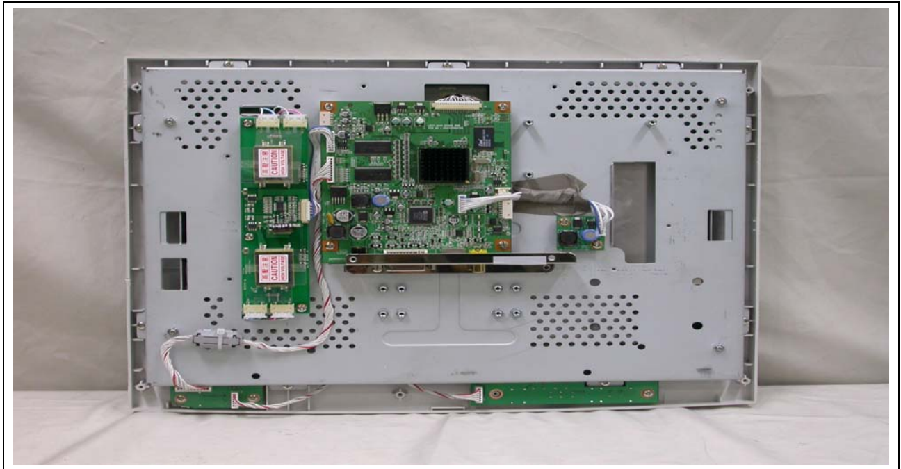
Figure 3 : Inner(NEC Panel)
