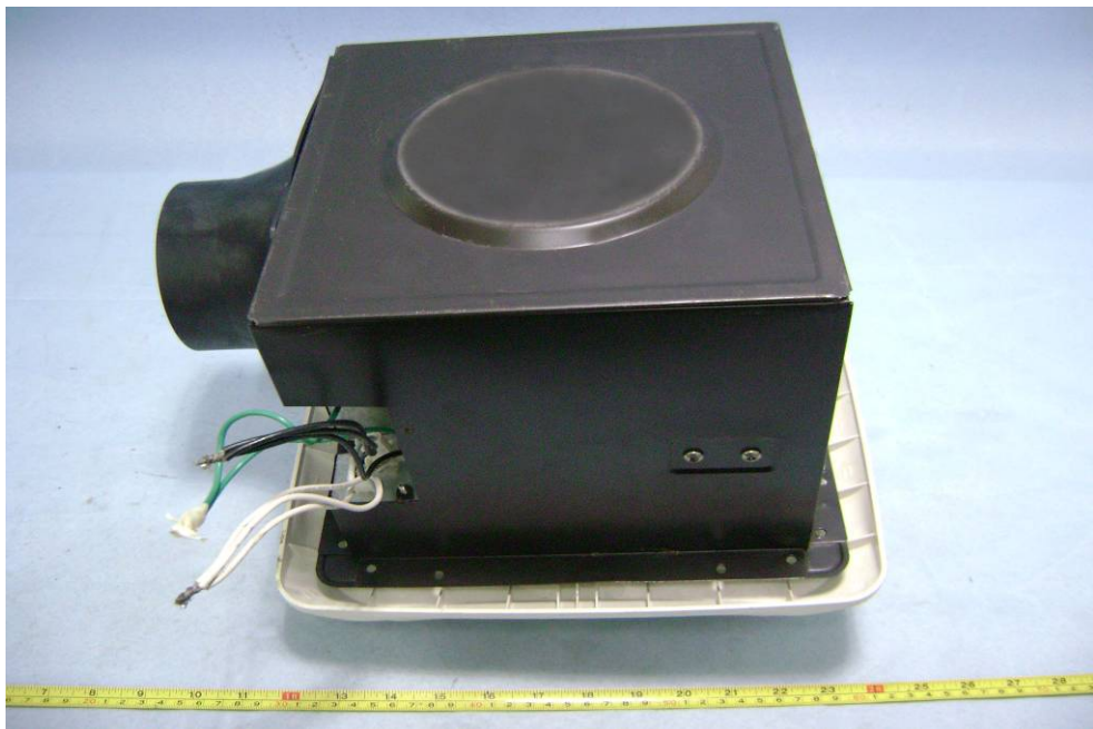
EUT with plastic chimney-Front View
