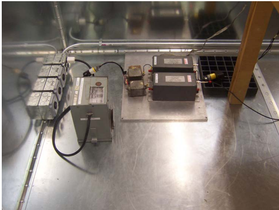
Conducted Emissions Test Setup, Measurement Location, Side View
