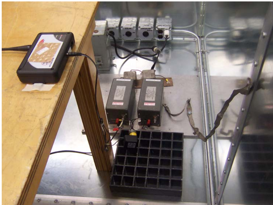
Conducted Emissions Test Setup, Measurement Location
