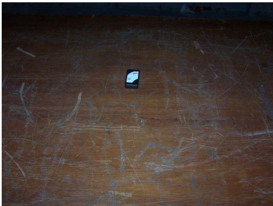
Radiated Emissions, Spurious Case, X-Axis Setup
