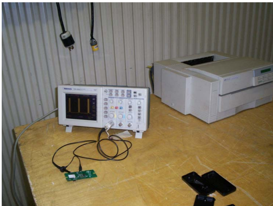
Duty Cycle Determination, Test Setup
