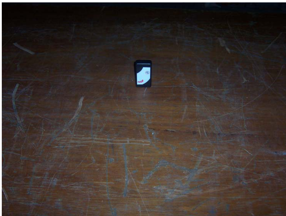
Radiated Emissions, Fundamental and Harmonics, Z-Axis Setup
