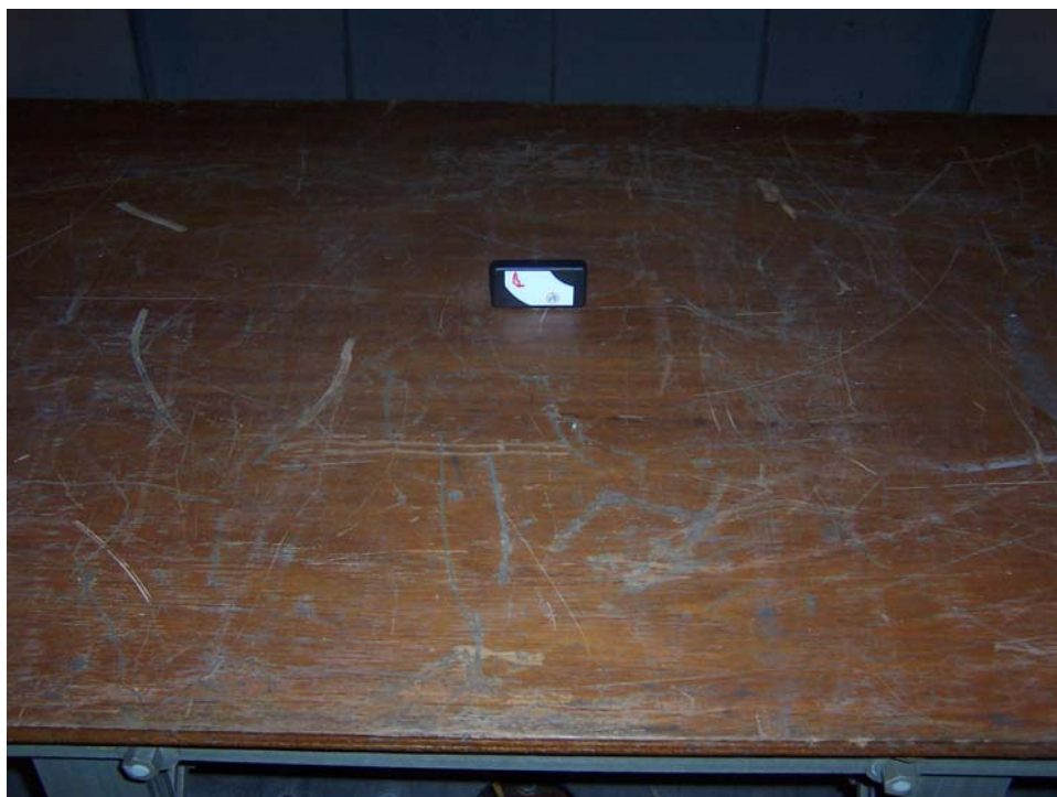
Radiated Emissions, Fundamental and Harmonics, Y-Axis Setup
