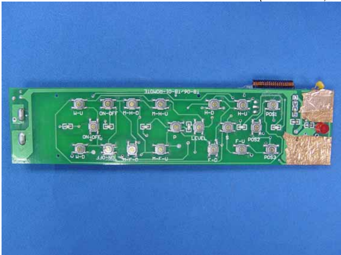
Figure 6 Internal View (Control Board, Back View)
