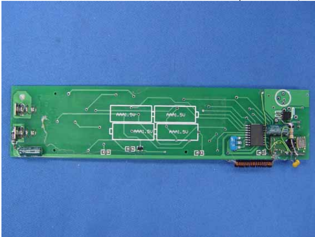
Figure 5 Internal View (Control Board, Front View)
