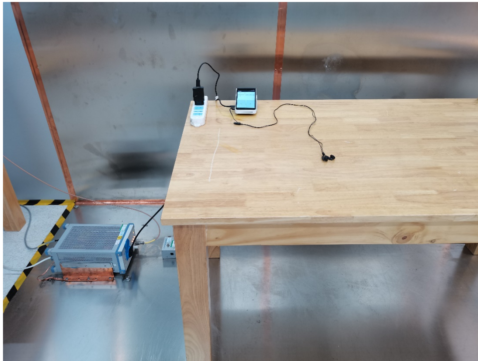
Photograph 1: Set-up photo for Conducted Emission
