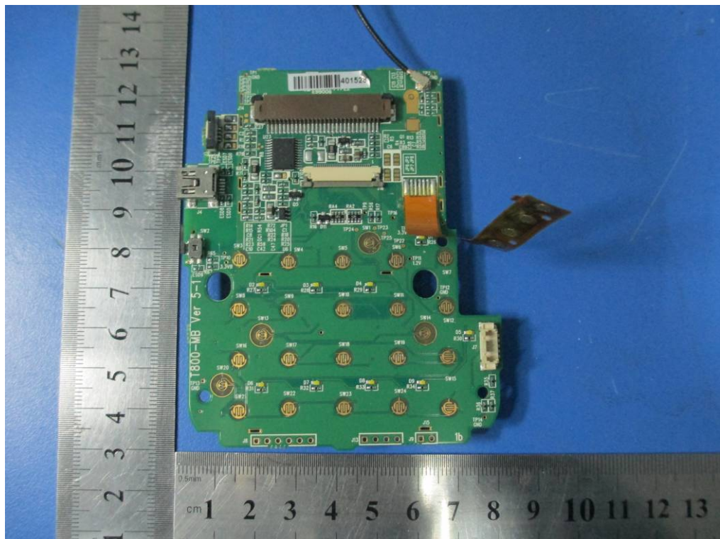
EUT PCB Board 3 - Bottom View
