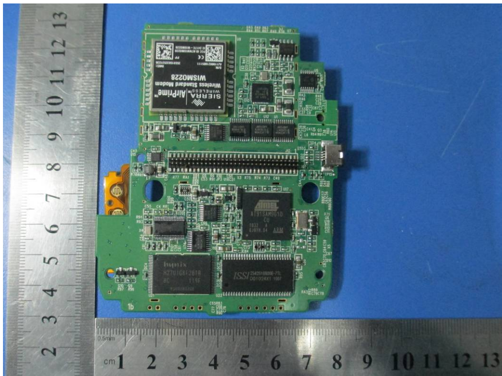
EUT PCB Board 3 - Top View
