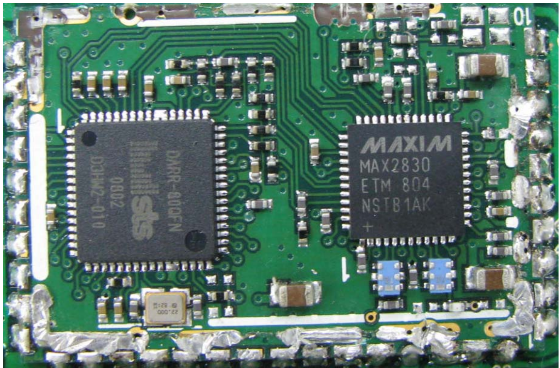
Figure 7-RF Module 1
