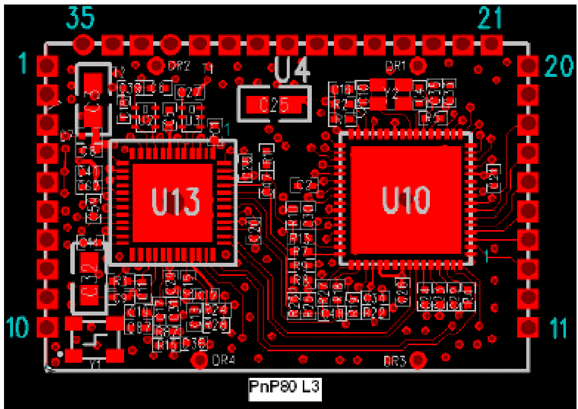
Figure 8-RF Module lay out
