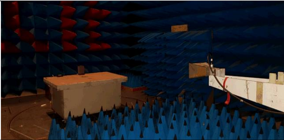
MEASUREMENT OF RADIATED DISTURBANCES ABOVE 1 GHz
