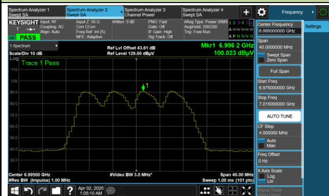
Channel 209 (6995MHz)
