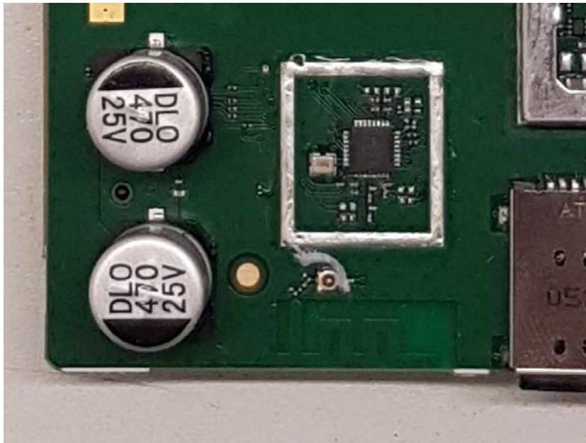
Photo 27 - BT antenna
