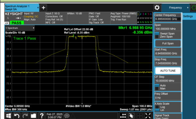
Channel 209 (6995MHz)
