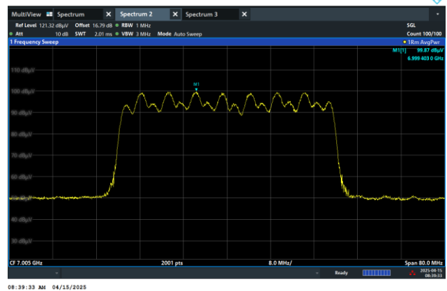
Channel 211 (7005MHz)
