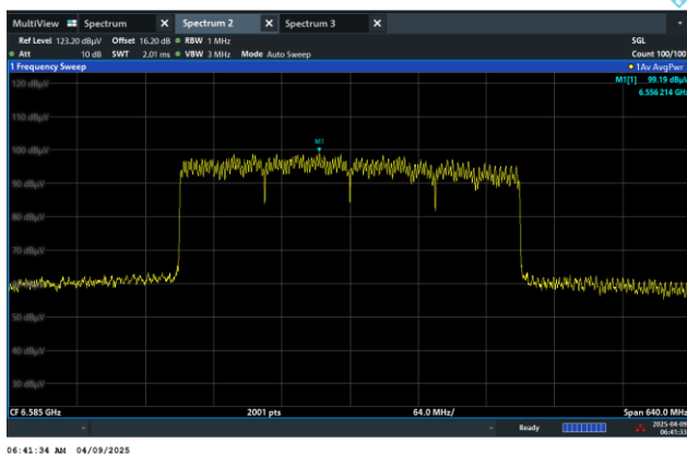
Channel 127 (6585MHz)
