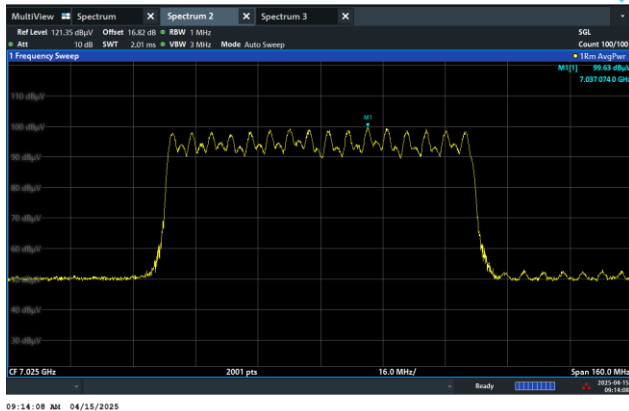
Channel 215 (7025MHz)
