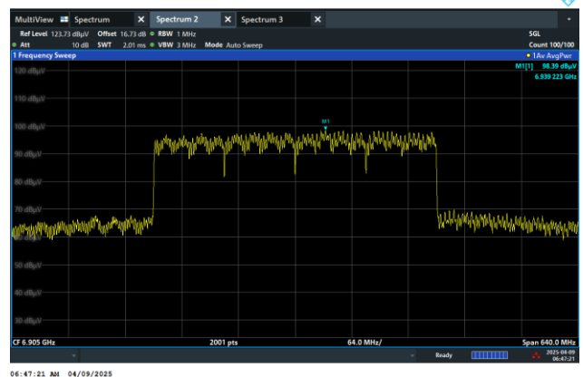
Channel 191 (6905MHz)
