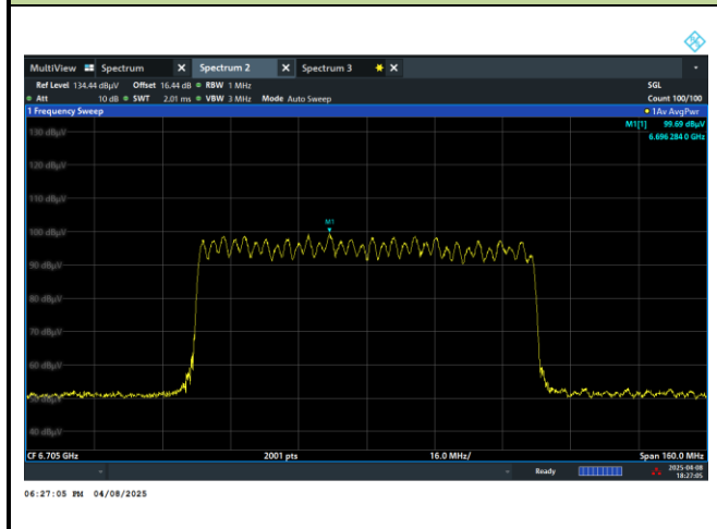
Channel 151 (6705MHz)
