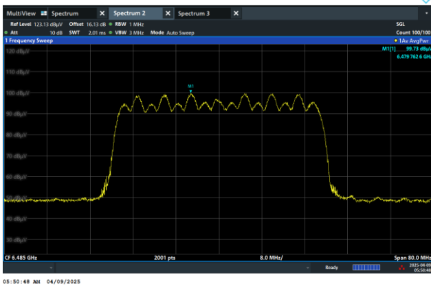
Channel 107 (6485MHz)
