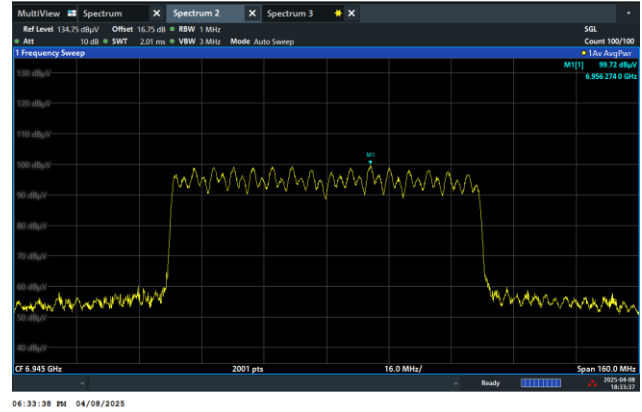
Channel 199 (6945MHz)
