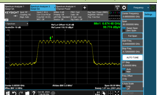
Channel 147 (6685MHz)
