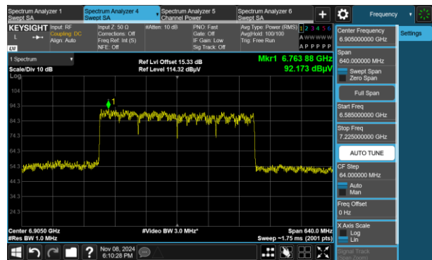
Channel 191 (6905MHz)
