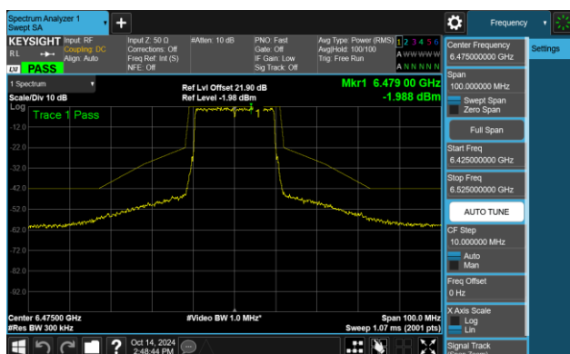
Channel 105 (6475MHz)
