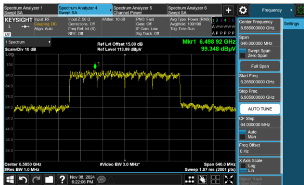
Channel 127 (6585MHz)
