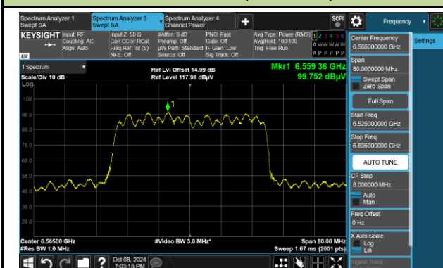
Channel 123 (6565MHz)
