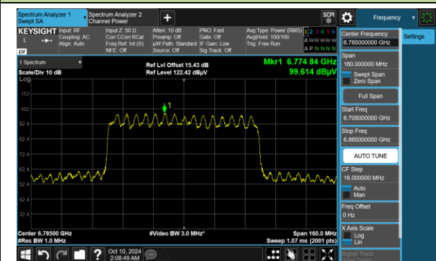
Channel 167 (6785MHz)
