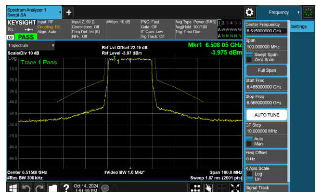
Channel 113 (6515MHz)
