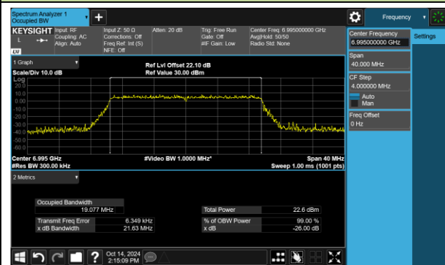
Channel 209 (6995MHz)
