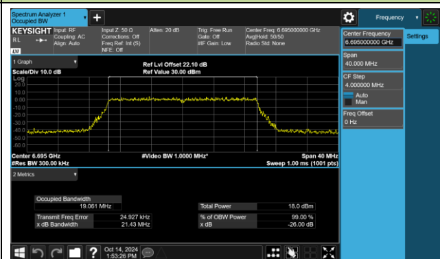
Channel 149 (6695MHz)
