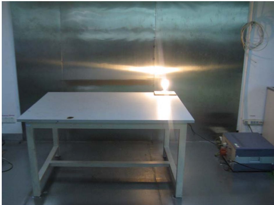
ESS-26W: Conducted Emissions - Side View
