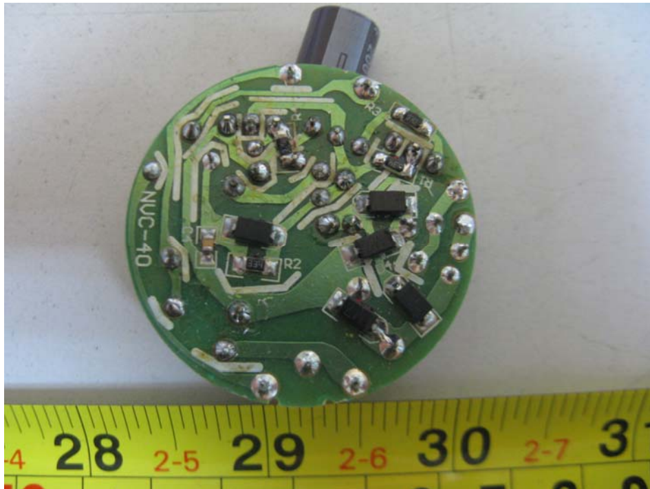
ESS-23W: EUT – Main Board Bottom View
