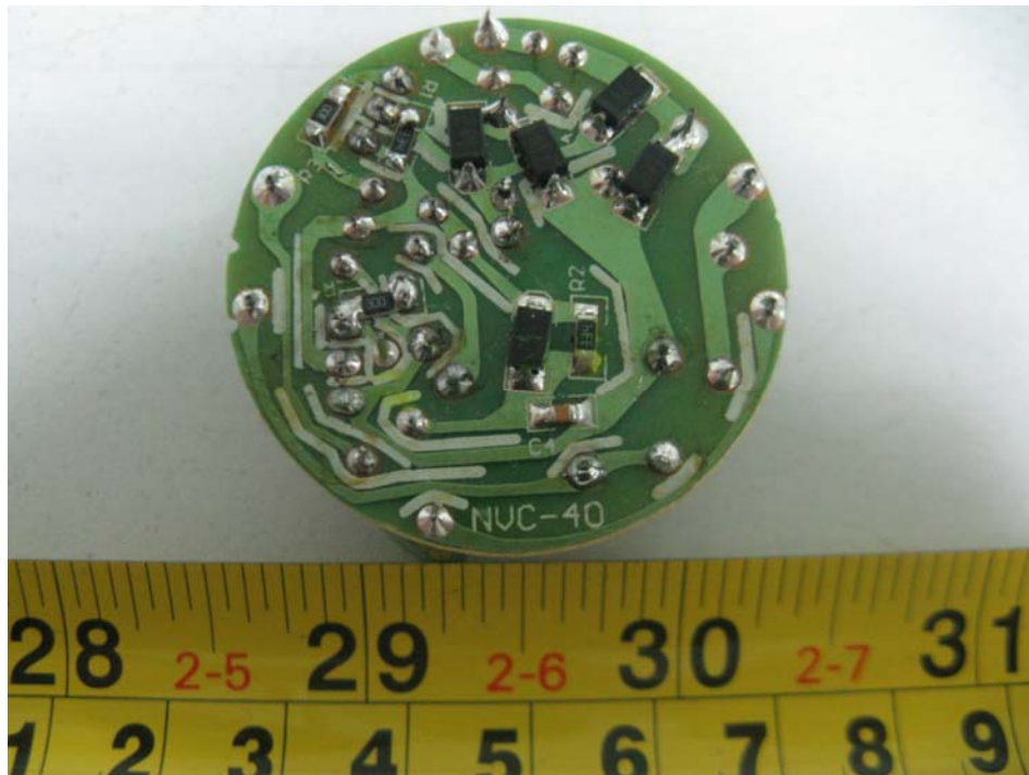
ESS-18W/20W: EUT – Main Board Bottom View
