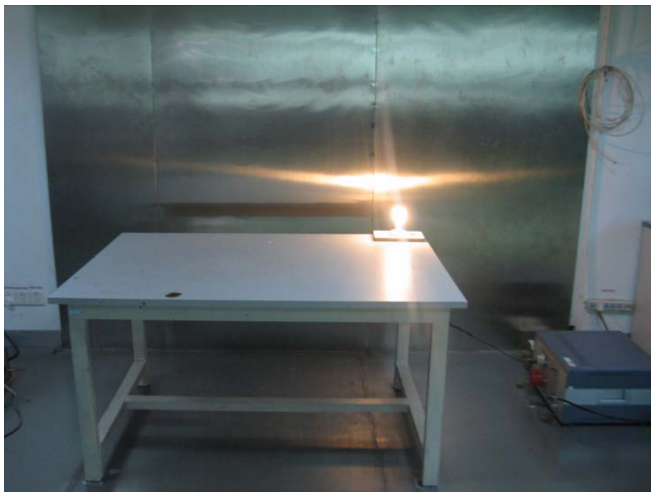
ESS-15W: Conducted Emissions - Side View
