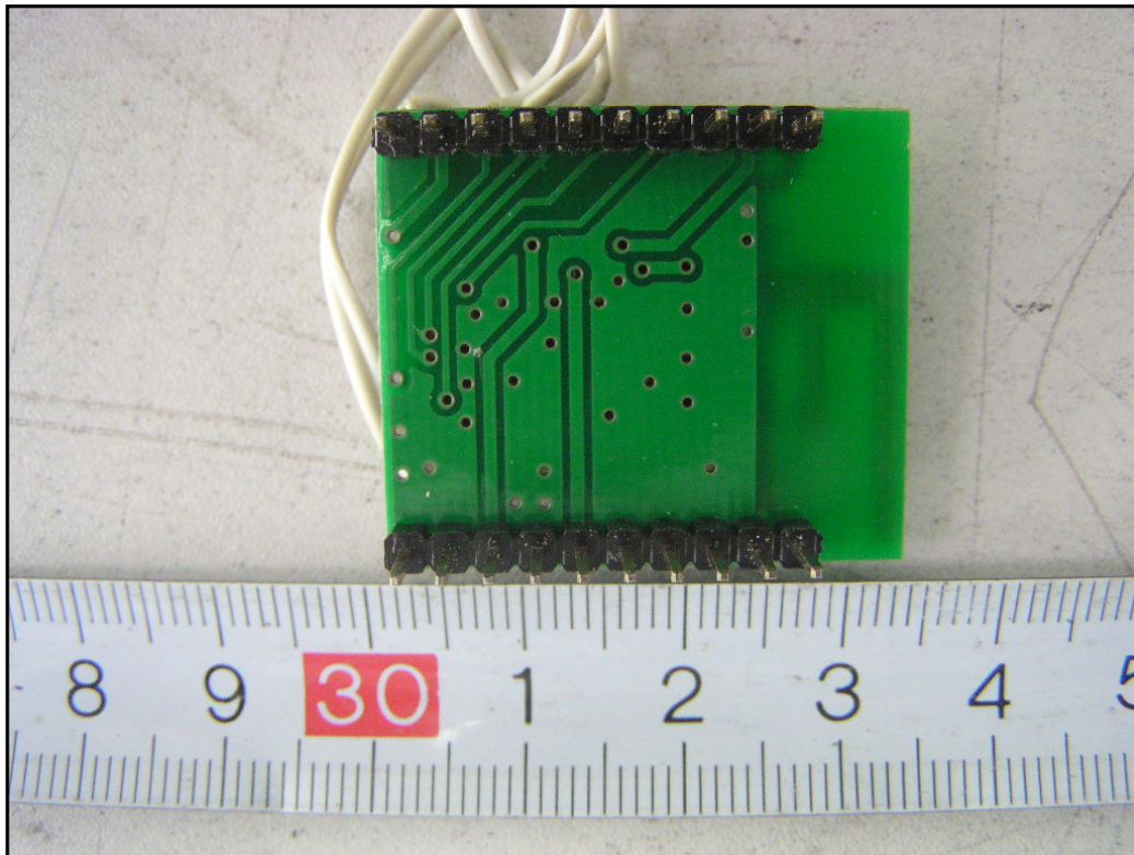
EUT – Bluetooth Board Circuit View
