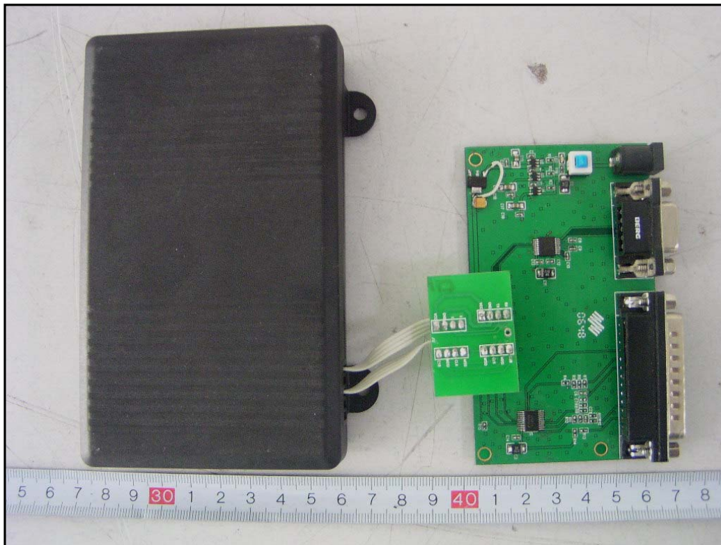
EUT and Test Board Front View
