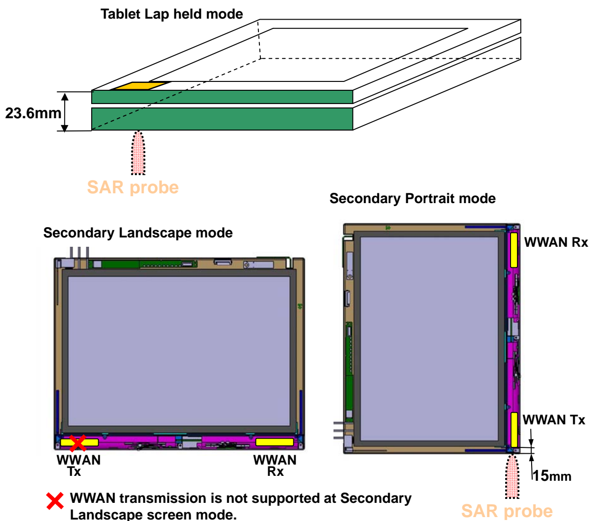
Figure 1 Antenna Locations
