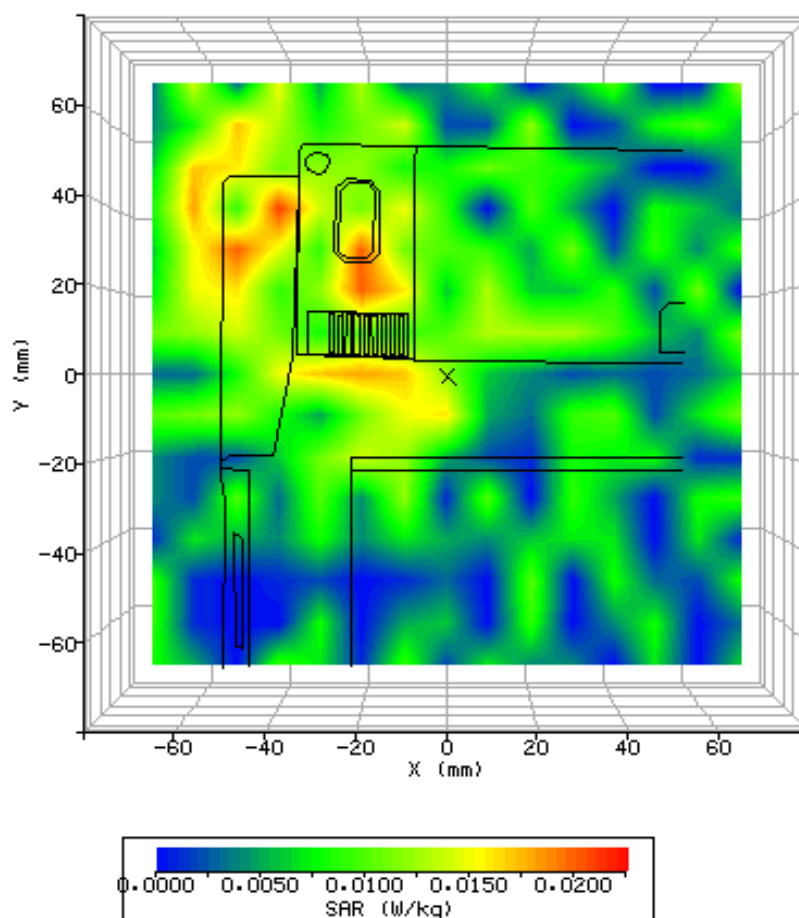
Figure 58: SAR Body Testing Results for the Ericsson Mobile Broadband Module in Screen 90° - Area 1 Phantom Position; Tested at 835MHz (FDDV Middle Channel) with 2mm Separation Distance to the Phantom (NUA).
