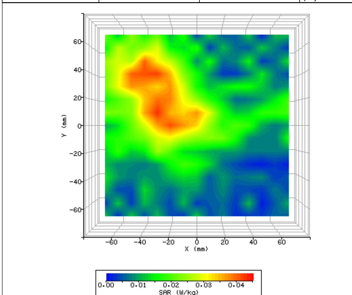
Figure 6: SAR Body Testing Results for the Ericsson Mobile Broadband Module in Screen 90° - Area 1 Phantom Position; Tested at 836.4MHz (GSM 850 Mid Channel) with 2mm Separation Distance to the Phantom (NUA).
