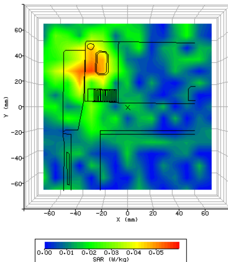
Figure 41: SAR Body Testing Results for the Ericsson Mobile Broadband Module in Screen 90° - Area 1 Phantom Position; Tested at 1922.6MHz (FDD I Low Channel) with 2mm Separation Distance to the Phantom (NUA).
