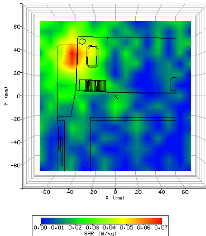
Figure 42: SAR Body Testing Results for the Ericsson Mobile Broadband Module in Screen 90° - Area 1 Phantom Position; Tested at 1922.6MHz (FDD I Low Channel) with 2mm Separation Distance to the Phantom (NUA).
