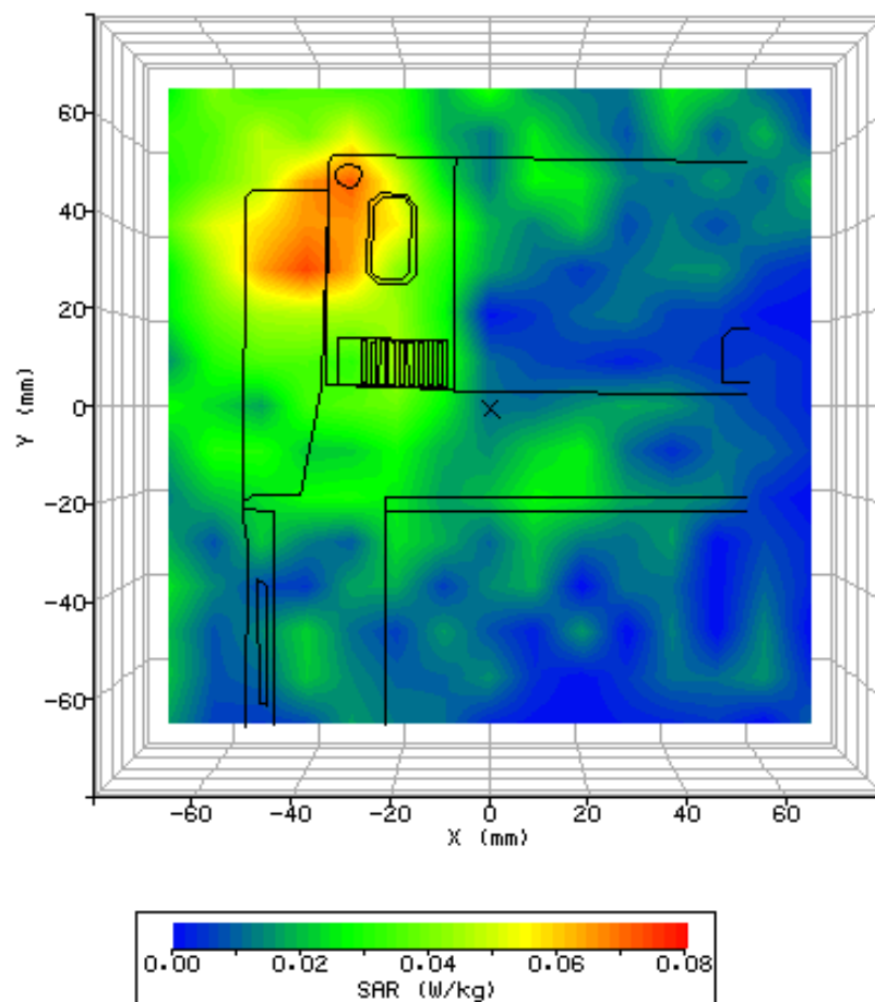
Figure 50: SAR Body Testing Results for the Ericsson Mobile Broadband Module in Screen 90° - Area 1 Phantom Position; Tested at 1880MHz (FDD II Mid Channel) with 2mm Separation Distance to the Phantom (NUA).
