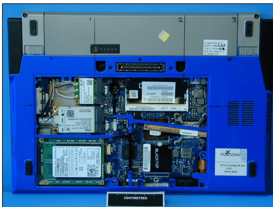
Figure 108: View of Modules in Laptop.
