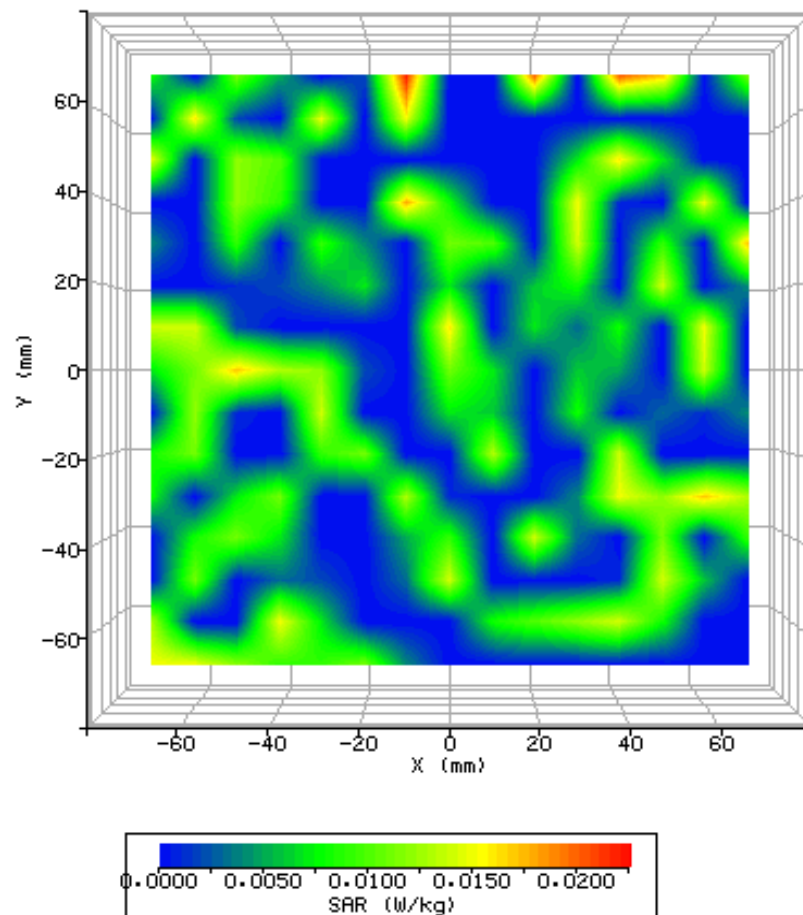
Figure 59: SAR Body Testing Results for the Intel WiFi Module in Screen 90° - Area 1 Phantom Position; Tested at 2412MHz (WLAN Low Channel) with 2mm Separation Distance to the Phantom (NUA).
