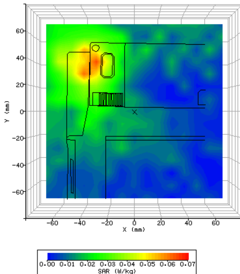
Figure 49: SAR Body Testing Results for the Ericsson Mobile Broadband Module in Screen 90° - Area 1 Phantom Position; Tested at 1880MHz (FDD II Mid Channel) with 2mm Separation Distance to the Phantom (NUA).
