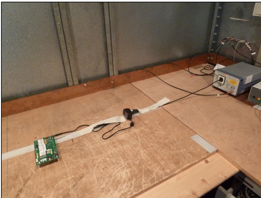
Photo 3: conducted emission
