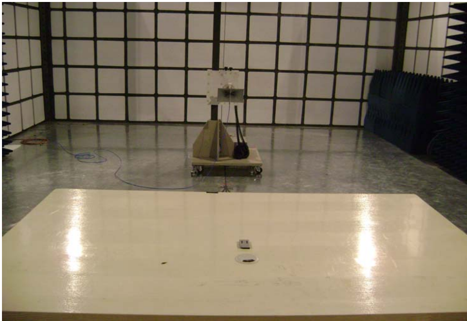
Radiation Emission Test View For 1GHz-4GHz
