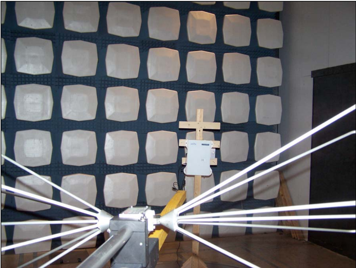
Photograph 3. Radiated Emissions, 30 MHz to 200 MHz
