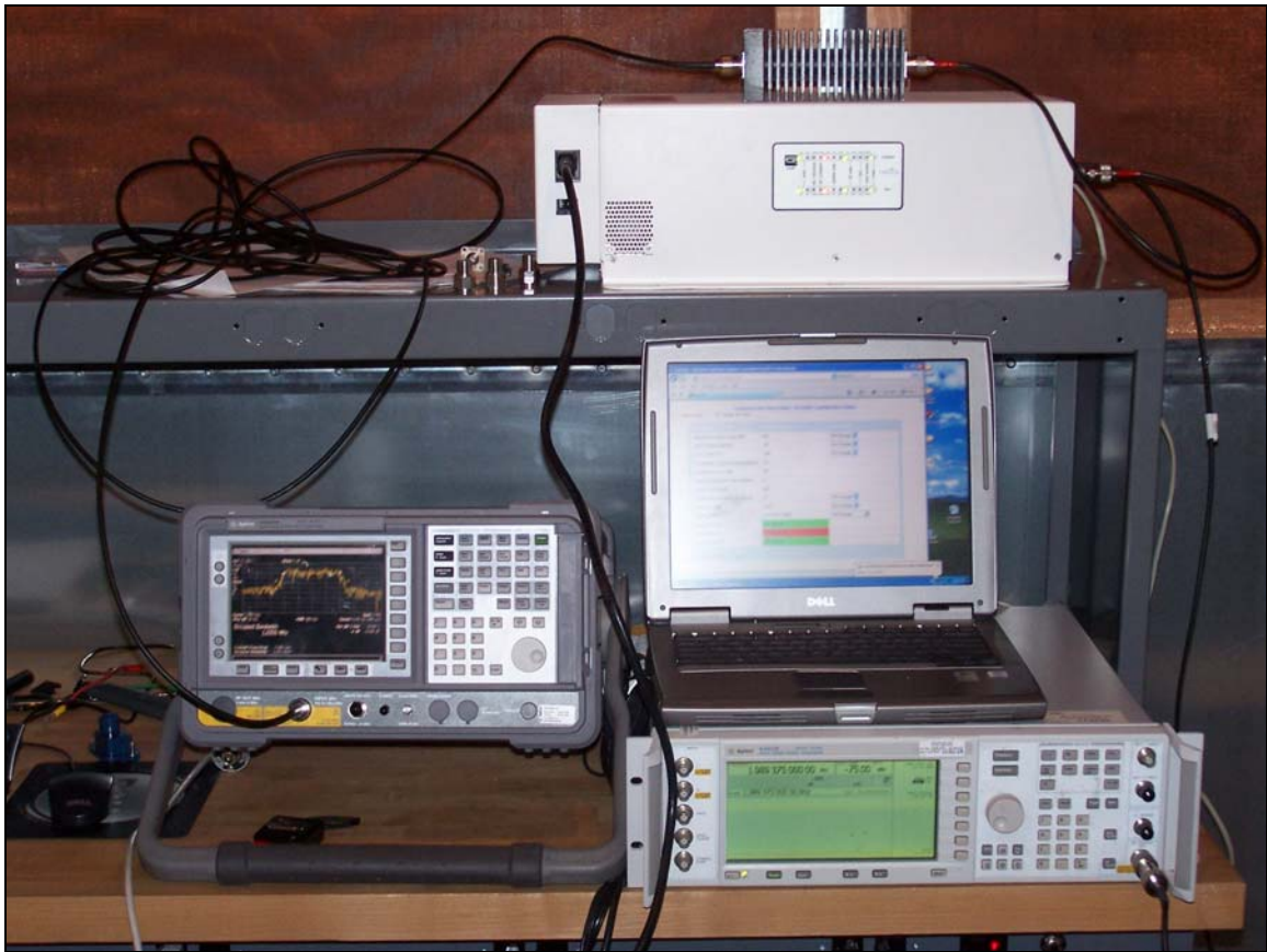
Photograph 2. Conducted Emissions Test Setup
