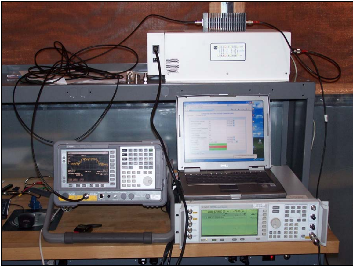
Photograph 4. Conducted Emissions Test Setup
