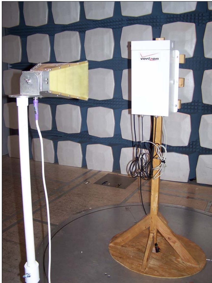
Photograph 5. Radiated Emissions Test Setup
