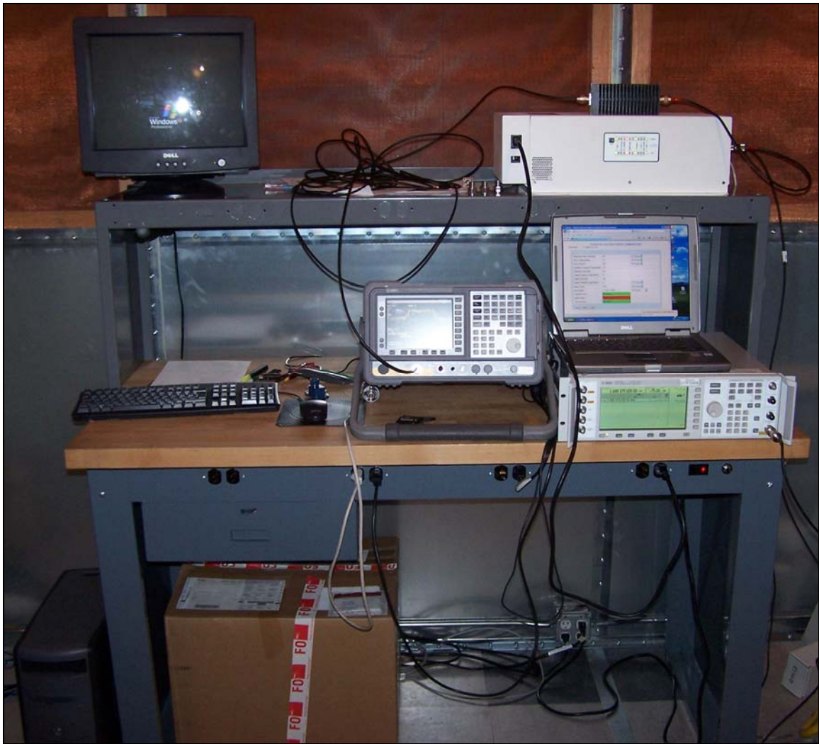
Photograph 3. Conducted Emissions Test Setup
