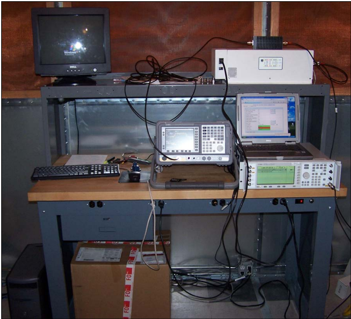
Photograph 1. Conducted Emissions Test Setup
