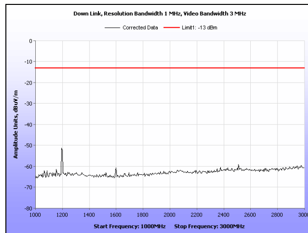
Plot 9. Radiated Spurious Emissions, Downlink, 1 GHz – 3 GHz
