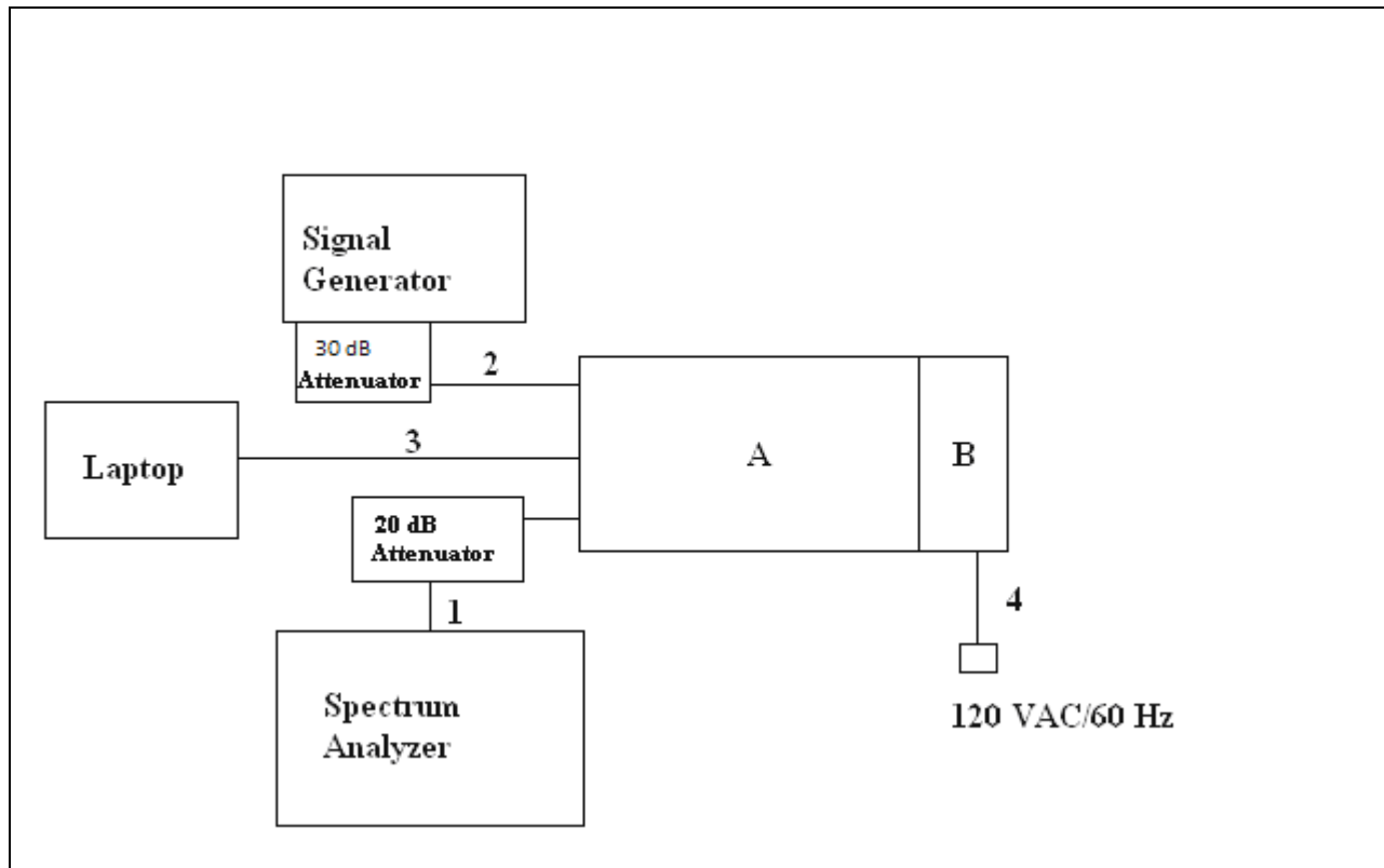
Figure 1. Block Diagram of Test Configuration (Conducted Measurement – Downlink)
