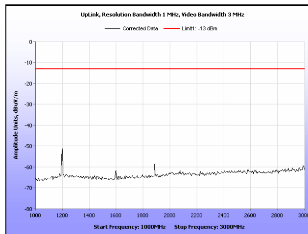
Plot 12. Radiated Spurious Emissions, Uplink, 1 GHz – 3 GHz
