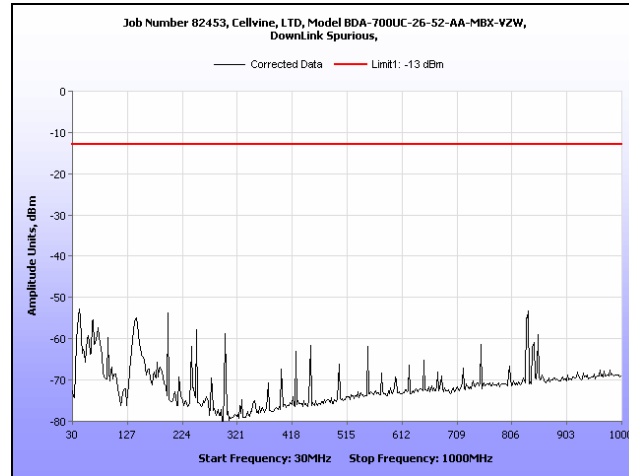
Plot 8. Radiated Spurious Emissions, Downlink, 30 MHz – 1 GHz
