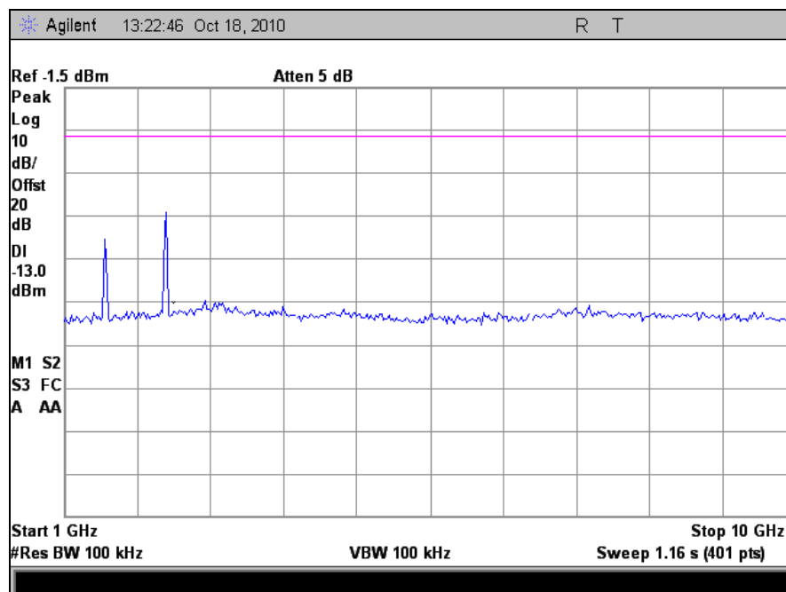
Plot 17. Conducted Spurious Emissions, Uplink, 1 GHz – 10 GHz
