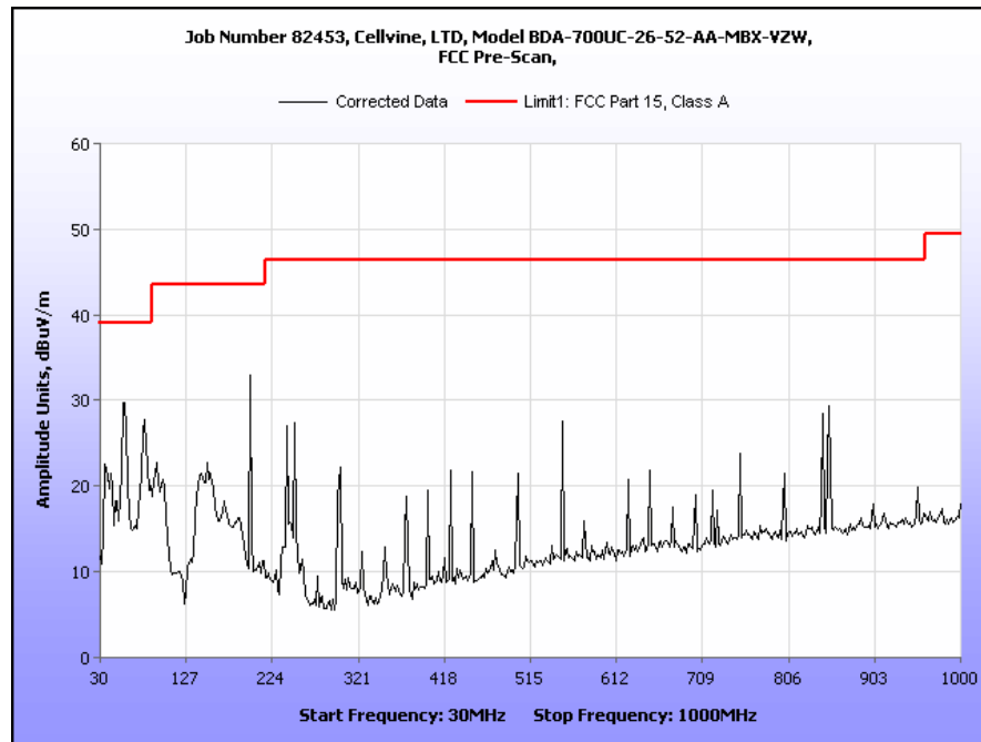
Plot 3. Radiated Emissions Limits, Pre-Scan
