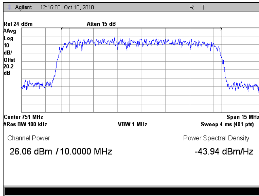
Plot 4. Output Power, Downlink
