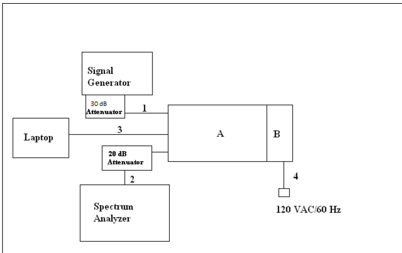
Figure 2. Block Diagram of Test Configuration (Conducted Measurement - Uplink)
