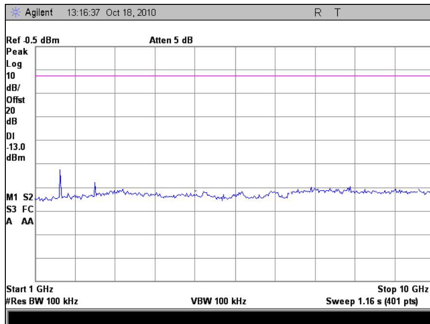
Plot 15. Conducted Spurious Emissions, Downlink, 1 GHz – 10 GHz
