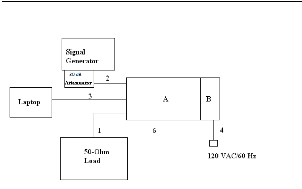
Figure 3. Block Diagram of Test Configuration (Radiated Measurement – Downlink)
