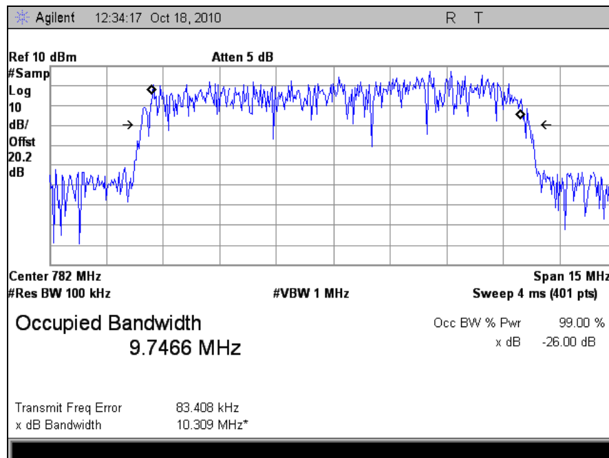
Plot 7. Occupied Bandwidth, Uplink
