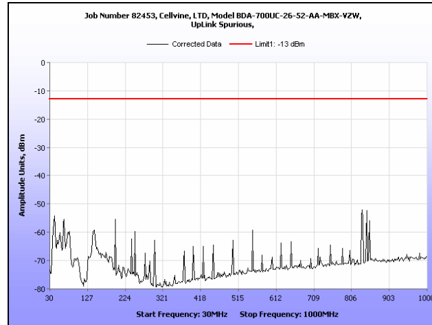
Plot 11. Radiated Spurious Emissions, Uplink, 30 MHz – 1 GHz
