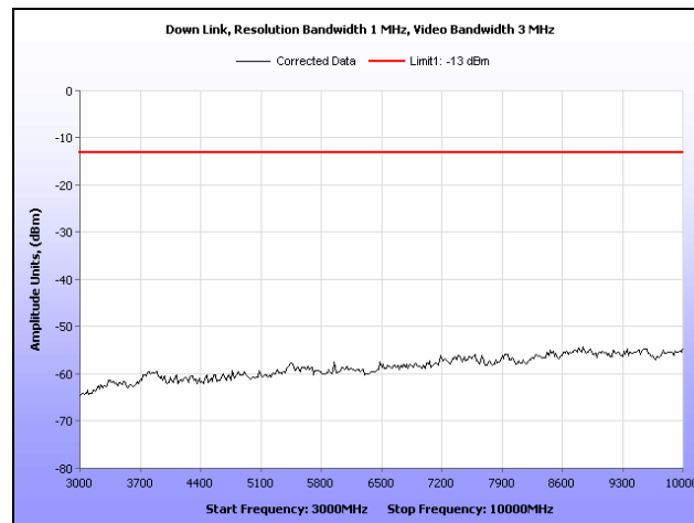
Plot 10. Radiated Spurious Emissions, Downlink, 3 GHz – 10 GHz
