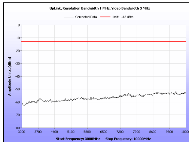
Plot 13. Radiated Spurious Emissions, Uplink, 3 GHz – 10 GHz
