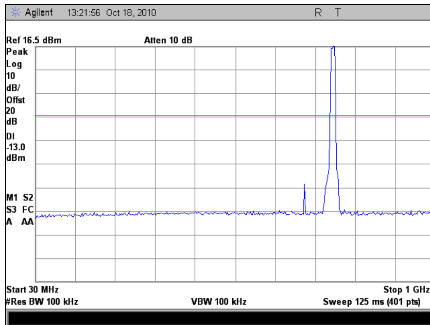
Plot 16. Conducted Spurious Emissions, Uplink, 30 MHz – 1 GHz
