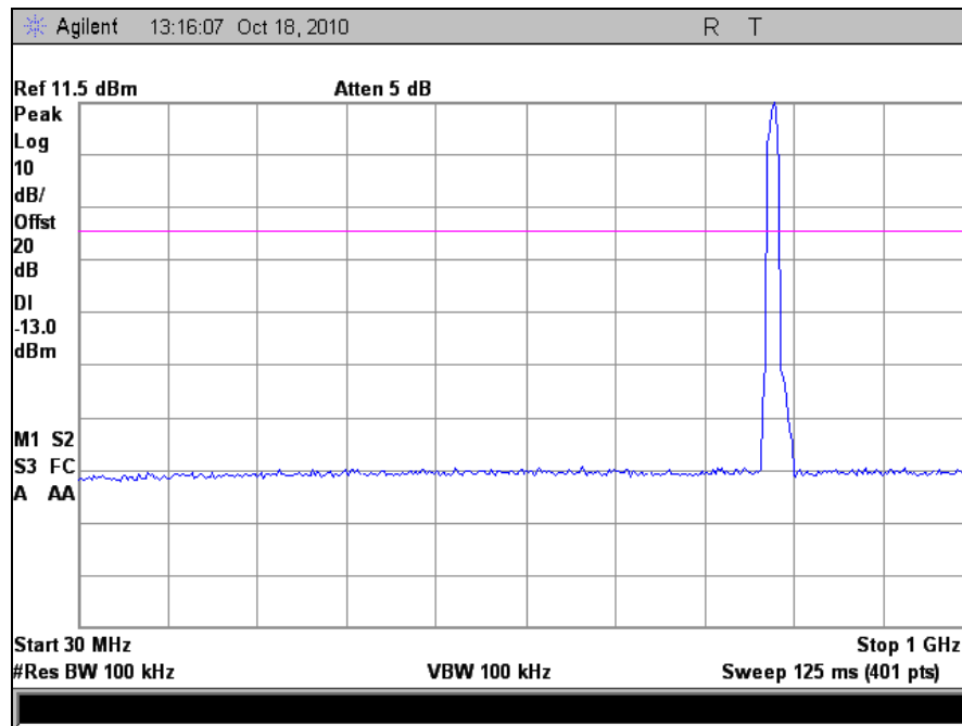
Plot 14. Conducted Spurious Emissions, Downlink, 30 MHz – 1 GHz
