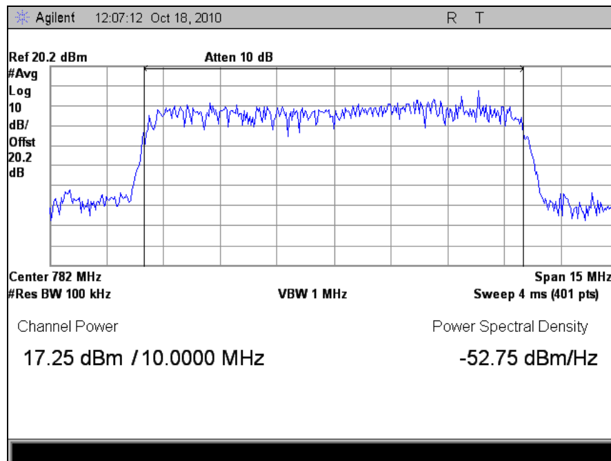
Plot 5. Output Power, Uplink
