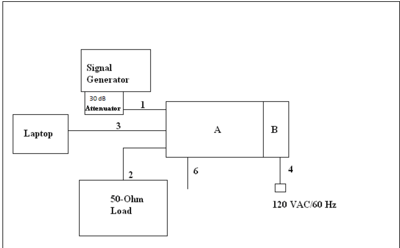
Figure 4. Block Diagram of Test Configuration (Radiated Measurement - Uplink)
