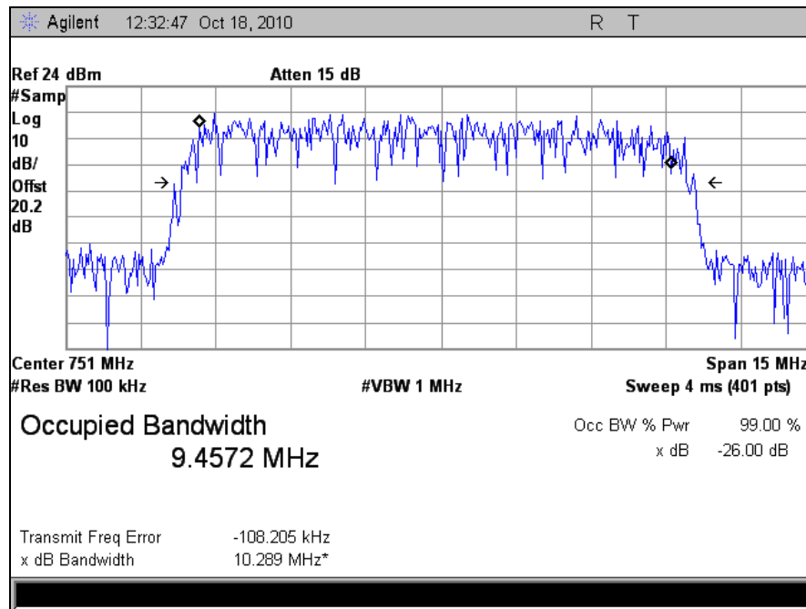
Plot 6. Occupied Bandwidth, Downlink
