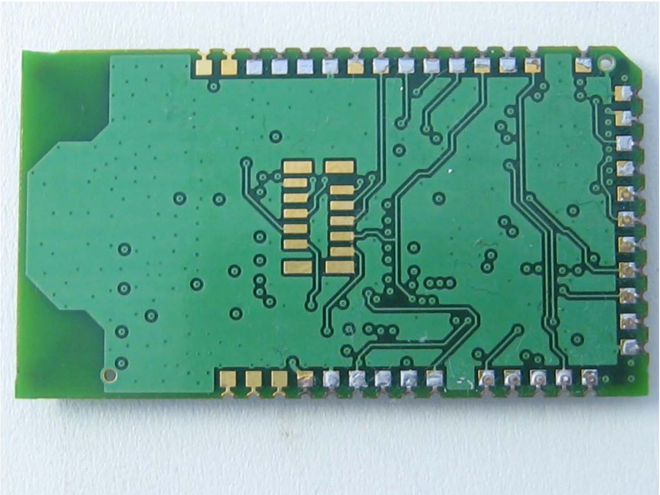
Healthsense MSR-11-200 Internal View BACK
